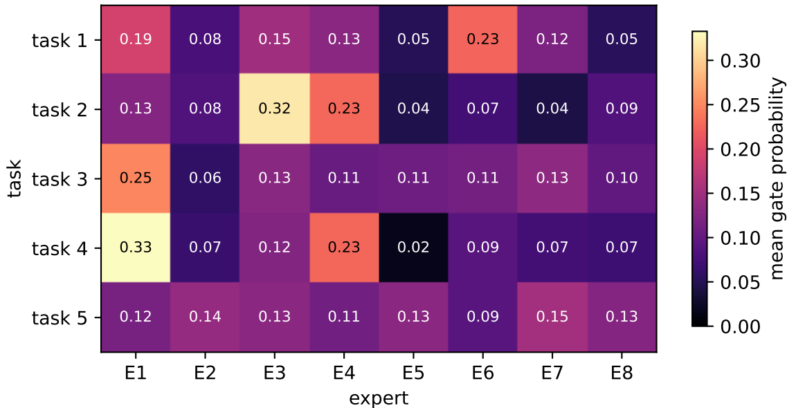
PermutedMNIST: input-level router profile (3 seeds)
