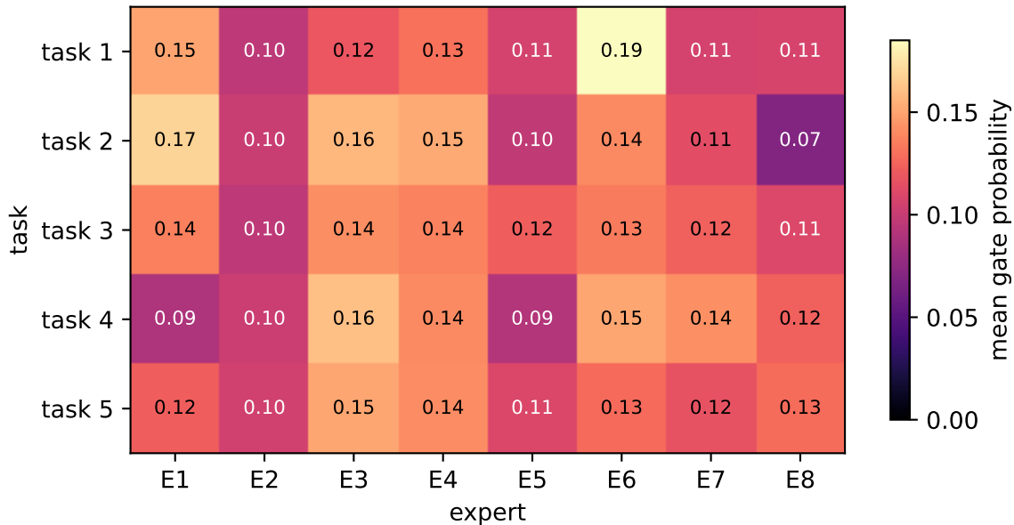
SplitMNIST: input-level router profile (3 seeds)
