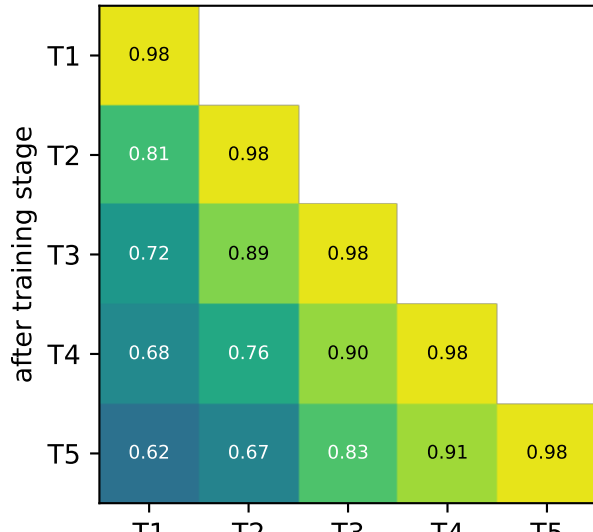
Naive MLP
