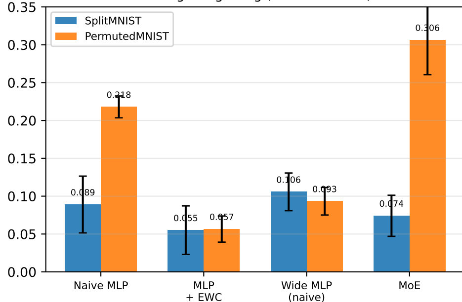
Average forgetting (lower is better)
