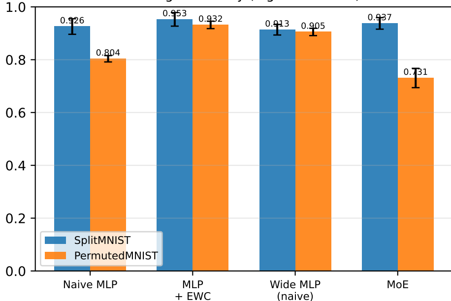
Average accuracy (higher is better)
