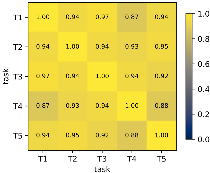
PermutedMNIST: routing similarity between tasks (cosine)
