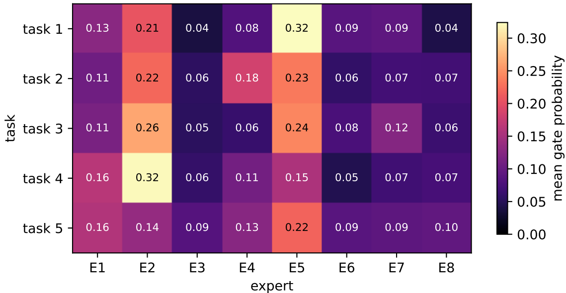
PermutedMNIST: mean gate probability per task and expert (3 seeds)
