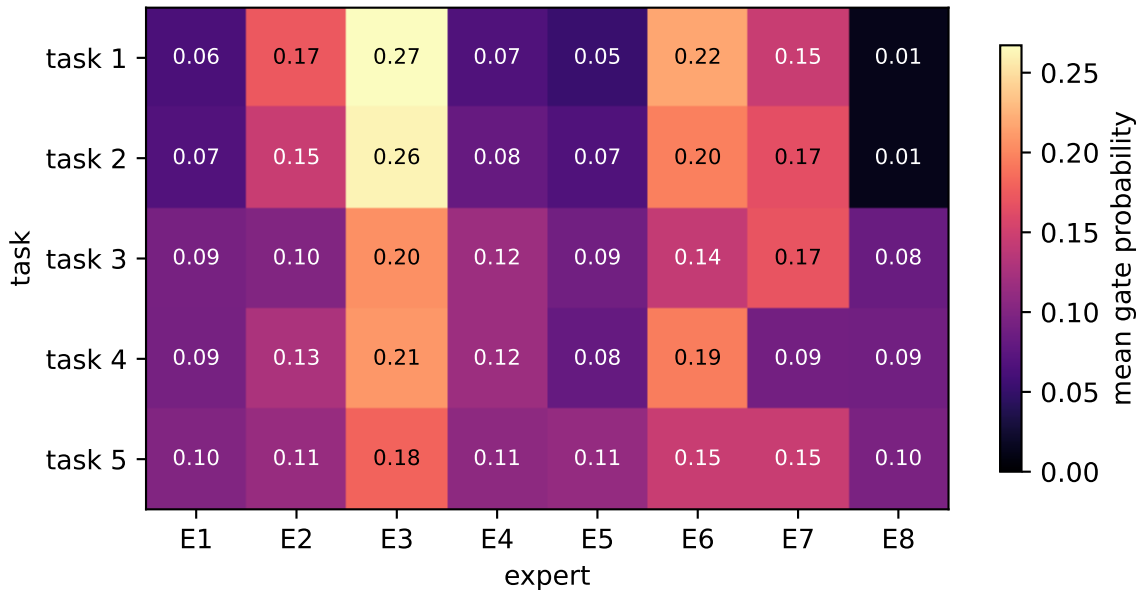
SplitMNIST: mean gate probability per task and expert (3 seeds)
