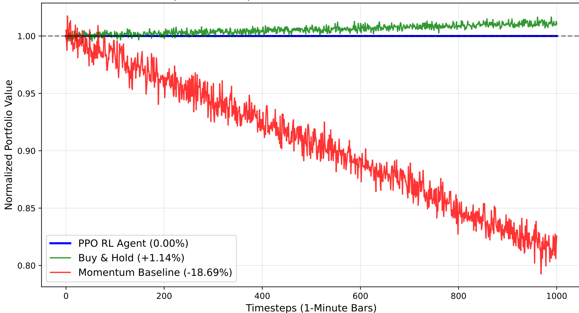
Figure 1: Cumulative Equity Curve Comparison (Impact of 1.0 bp Transaction Costs on 1-Minute Data)
