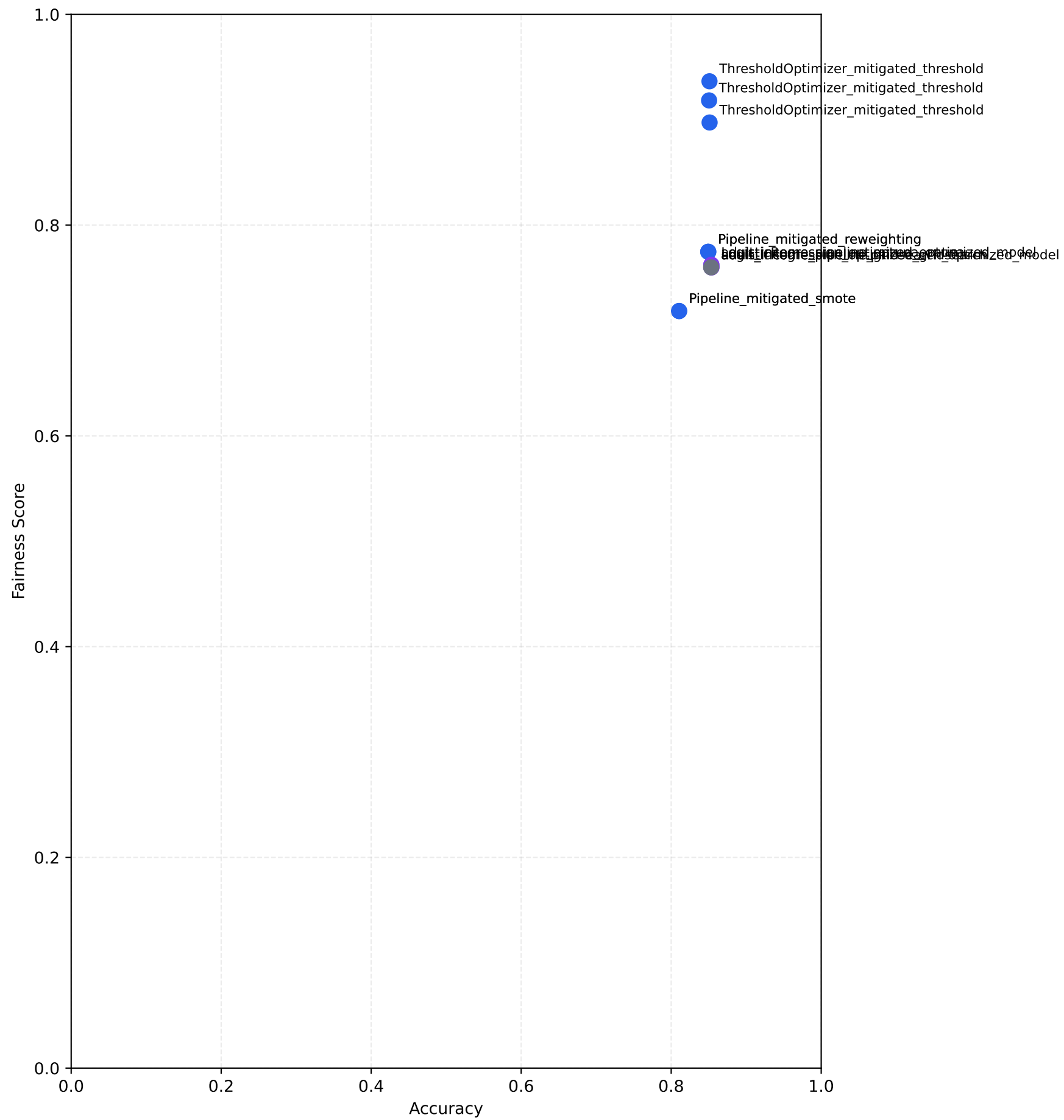
Accuracy vs Fairness Trade-off
