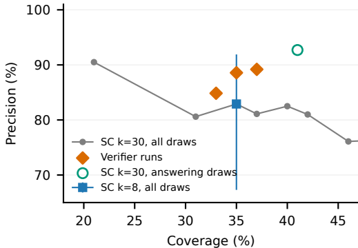
(b) Verifier and self-consistency
