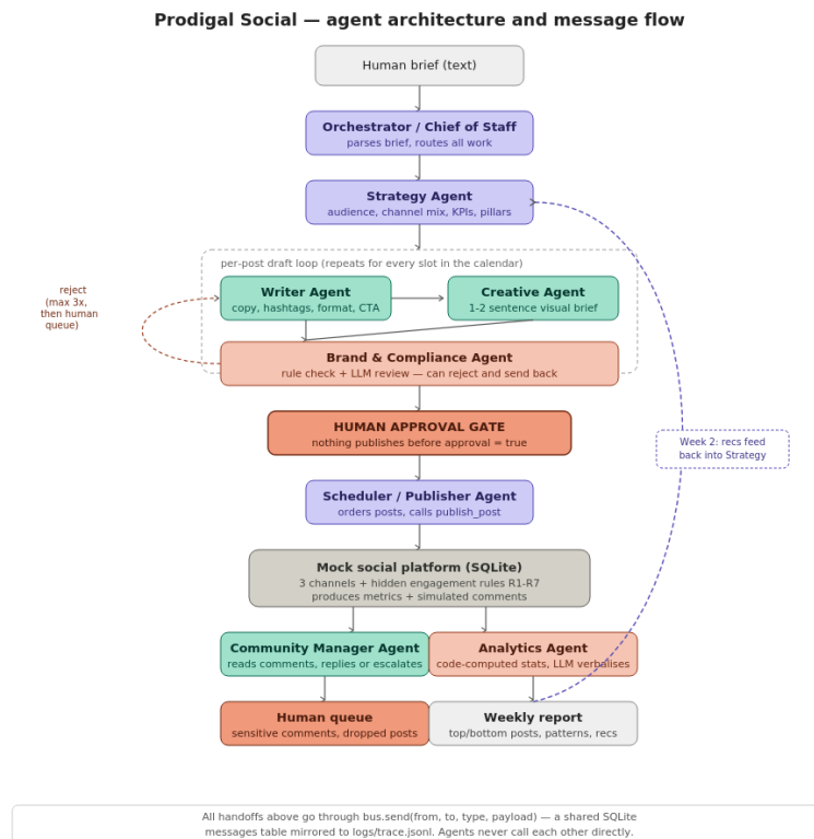
Agent organisation and message flow.
