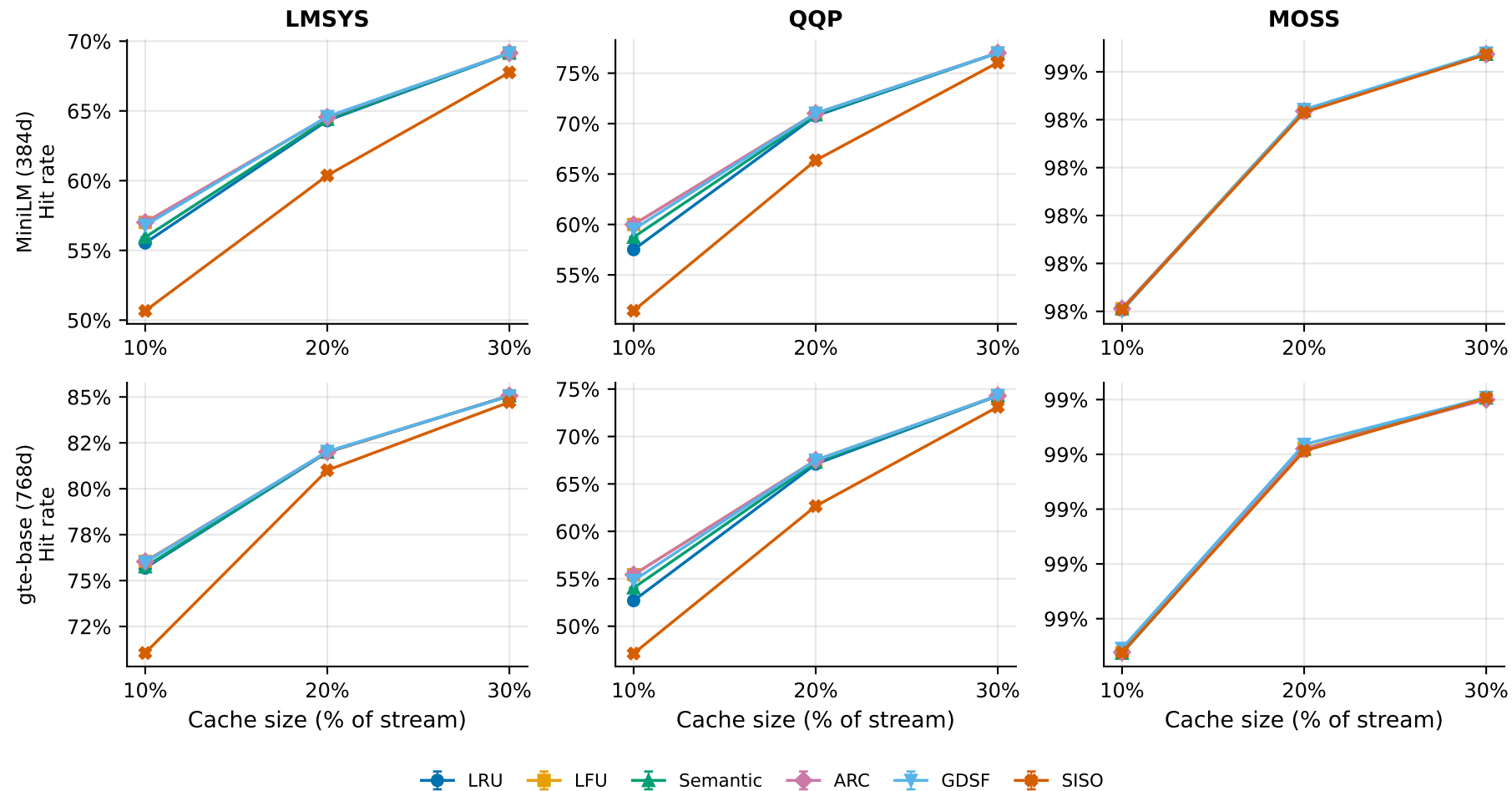
Phase 6 cache-size ablation — negative result replicates across encoders (absolute hit rates are not comparable across encoders; per-encoder hit-threshold calibration)
