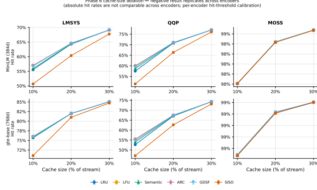
Figure 5: Cache-size ablation. Hit rate is governed by capacity, not policy: all policy gaps, including SISO’s deficit and LFU’s lead over LRU, shrink monotonically as the cache grows. The ordering replicates across both embedding encoders.
