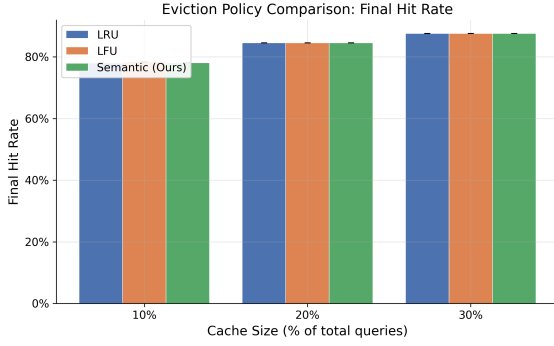
Figure 3: Hit rate across eviction policies at three cache capacities. All three policies converge to statistically equivalent performance.
