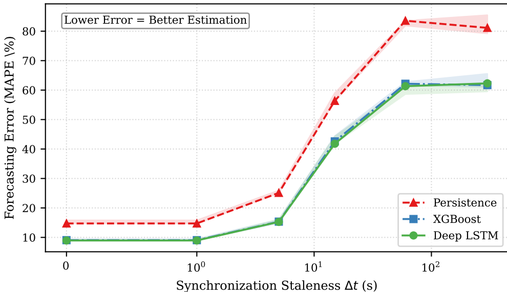
Short-Term Load Estimation Degradation vs. Staleness
