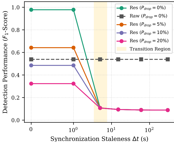
(a) LSTM Autoencoder
