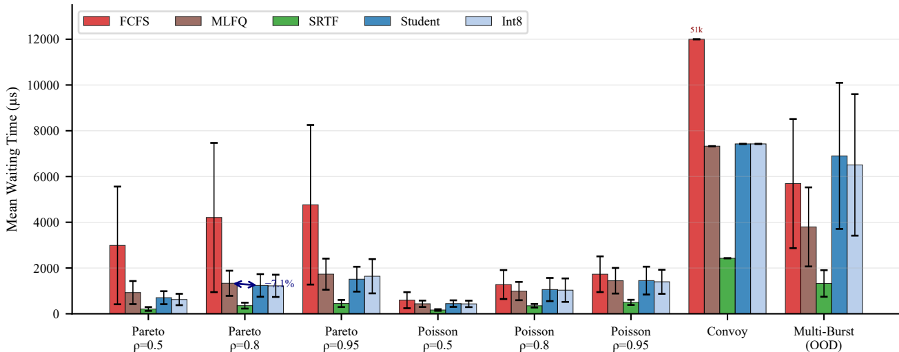
Policy Comparison Across Canonical Workloads (30-seed mean \pm 95% CI; Convoy bars clipped at 12 000 \mu s)
