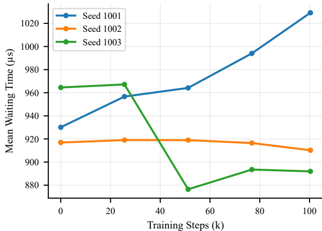
Student BC+PPO — Poisson \rho=0.8
