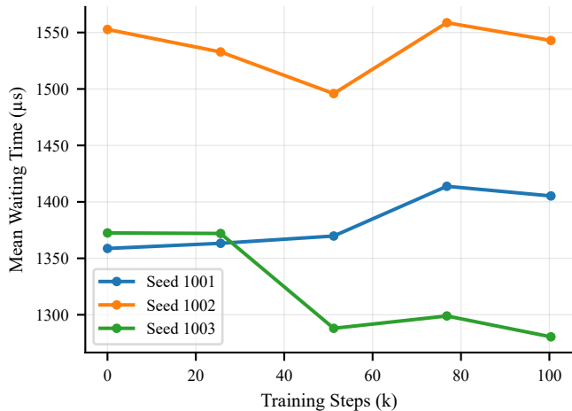
Student BC+PPO — Pareto \rho=0.8
