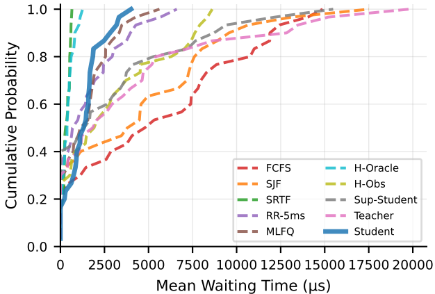
CDF of Mean Waiting Time (Pareto \rho=0.8 , 30 seeds)
