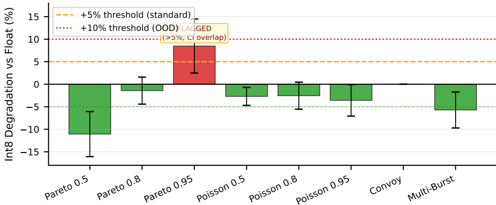
Int8 Quantization Degradation per Workload (positive = Int8 worse, negative = Int8 better)
