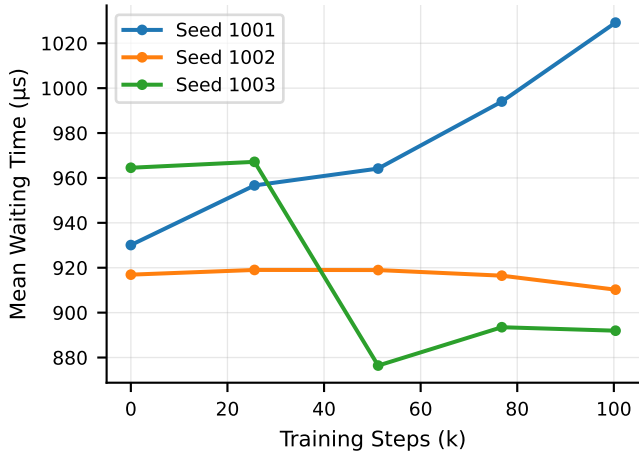
Student BC+PPO — Poisson \rho=0.8
