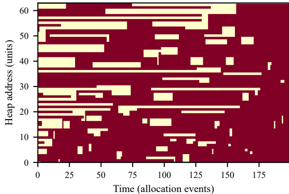
Best-Fit (Fragmented)
