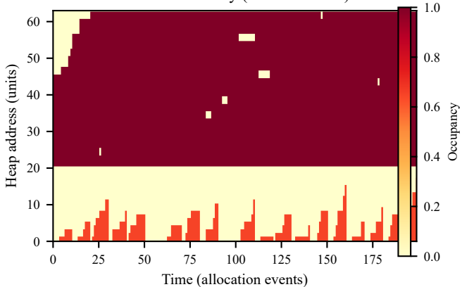
Lifetime-Affinity (NeuroOS-Lite)
