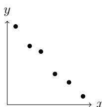
Strong Negative ( r \approx -1 )
