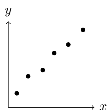
Strong Positive ( r \approx +1 )
