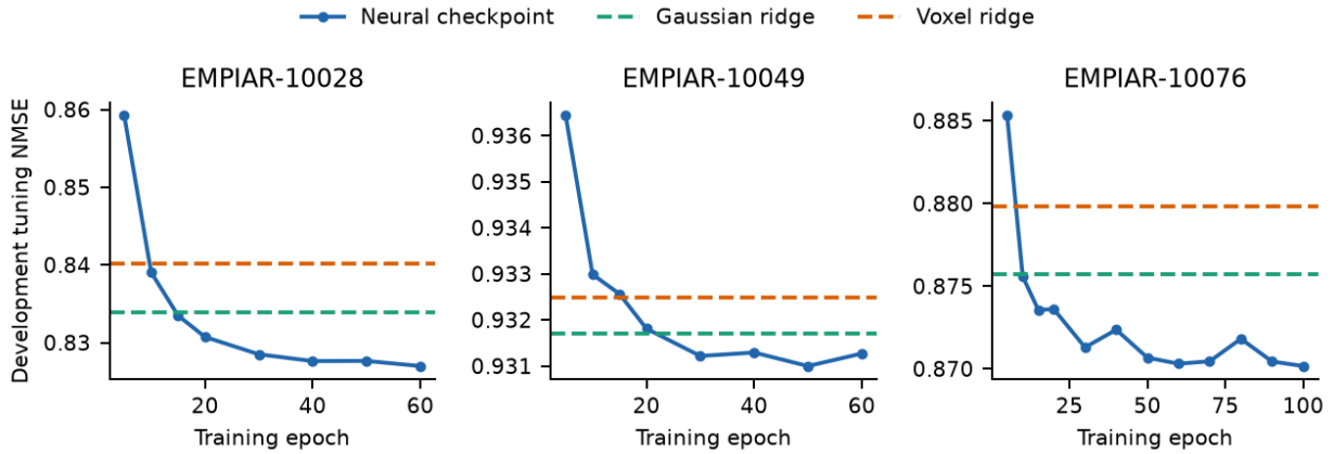
Figure 16. Development tuning error at all evaluated neural checkpoints, with the classical reconstruction controls. Checkpoint selection minimizes this tuning error; the test-group error is not used to select the checkpoint. Different training objectives and supplied consensus poses limit this comparison.
