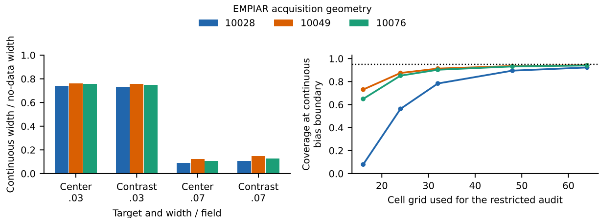
Figure 11. Left: optimized continuous fixed-pose widths for the full cube class. Right: cell-projected audit coverage at a constructed continuous bias boundary, for the broad central target and cell-fitted estimator. Reference-map coverage is one in these cases. The two panels answer distinct questions: useful width and omitted continuous directions.
