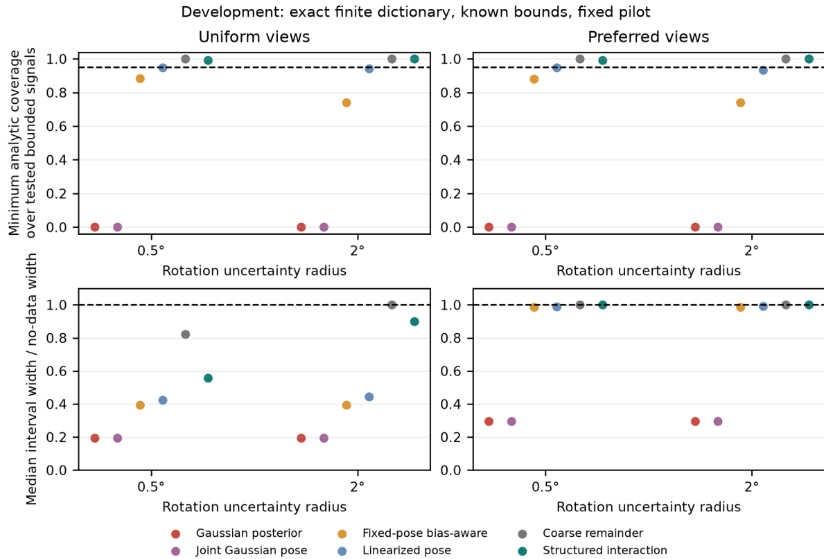
Figure 14. Exact-dictionary development tests with known bounds and an independent fixed pilot. Minimum coverage is over the finite tested set, including adversarial signals; it is not an empirical proof of the worst case. Widths count each independent design once. Gaussian posterior methods separately pass their correctly matched prior-predictive coverage check at 0.95. Their fixed-parameter boundary failures do not contradict Bayesian prior-average calibration.
