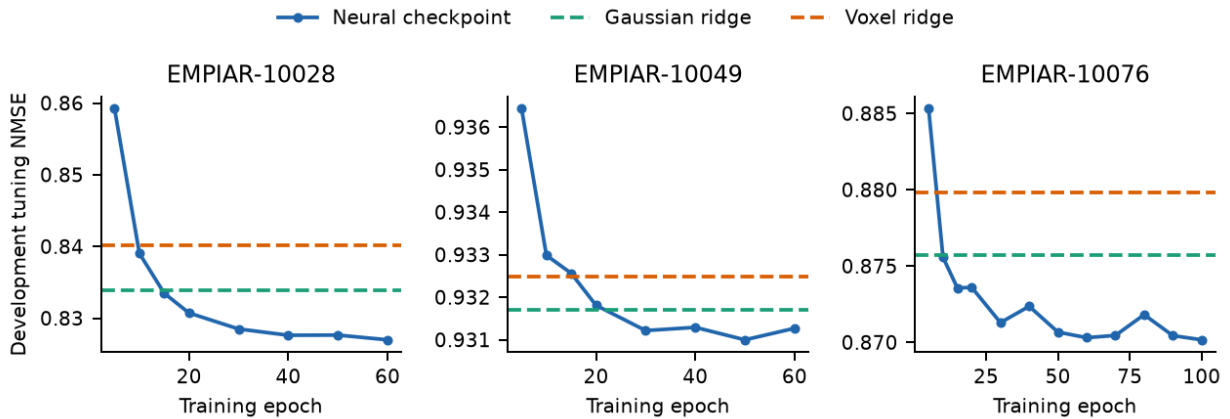
Figure 17. Development tuning error at all evaluated neural checkpoints, with the classical reconstruction controls. Checkpoint selection minimizes this tuning error; the test-group error is not used to select the checkpoint. Different training objectives and supplied consensus poses limit this comparison.
