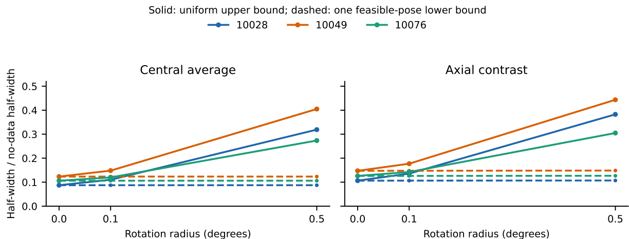
Figure 12. Continuous-density and nonlinear-pose development audit at target width 0.07 of the field. Solid curves are uniform conditional upper bounds for the same fixed-pose-optimized weights. Dashed curves use exact density-ball elimination at one allowed coherent rotation, providing feasible lower bounds on the required width, not global pose optima. Zero is the separate exact-pose control; the nonzero budgets also allow shifts of 0.01/24 field units. The visible gap exposes conservatism.
