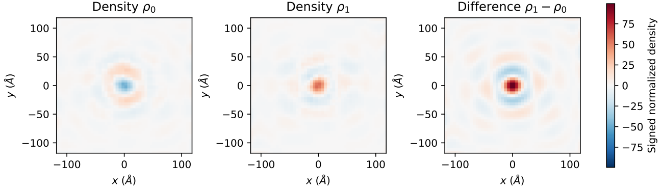
Figure 3. A continuous testing witness after the first alternating pose/density refit on 10049, displayed as 48-cell averages of the two central slices. The common color scale is symmetric and clipped. These are constructed signed densities in the declared mathematical class, not experimental reconstructions or a pair asserted to be molecular structures. Their allowed poses and whitened image-mean distance yield the conditional fixed-length lower bound; the displayed projections are for visualization only.
