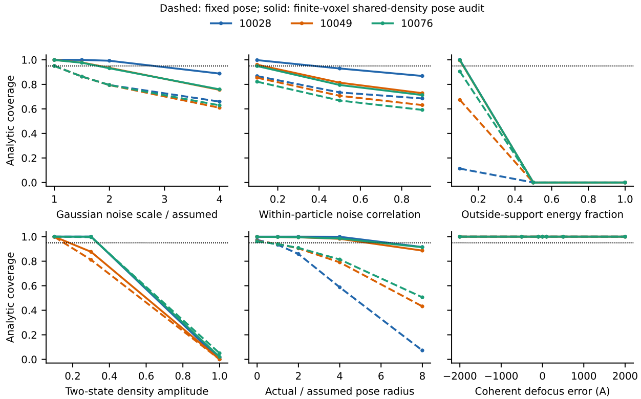
Figure 13. Deliberate assumption stresses for the finite-voxel central target. Curves share a signal within each geometry/control: the fixed-pose boundary for noise tests, a fixed-pose-estimator-directed support or mixture perturbation, or a saved nonlinear pose adversary. Dashed curves are fixed-pose certificates; solid curves include the shared-density pose audit. These are constructed diagnostic conditions, not experimental failure rates. All other controls remain in the result records.
