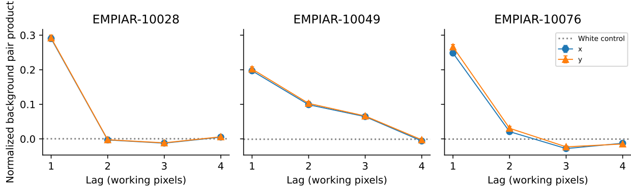
Figure 10. Descriptive background dependence in every additional-exposure image, after Fourier cropping of the downloaded particles to the working grid and before reconstruction windowing. We center and scale each image using pixels outside radius 0.43 of the box, then average products of background pixel pairs separated by each lag. Error bars are marginal 95% whole-exposure bootstrap intervals. Dotted lines show matched-statistic white-Gaussian controls. Background contamination and preprocessing prevent interpreting these values as pure-noise correlations or a confidence calibration.
