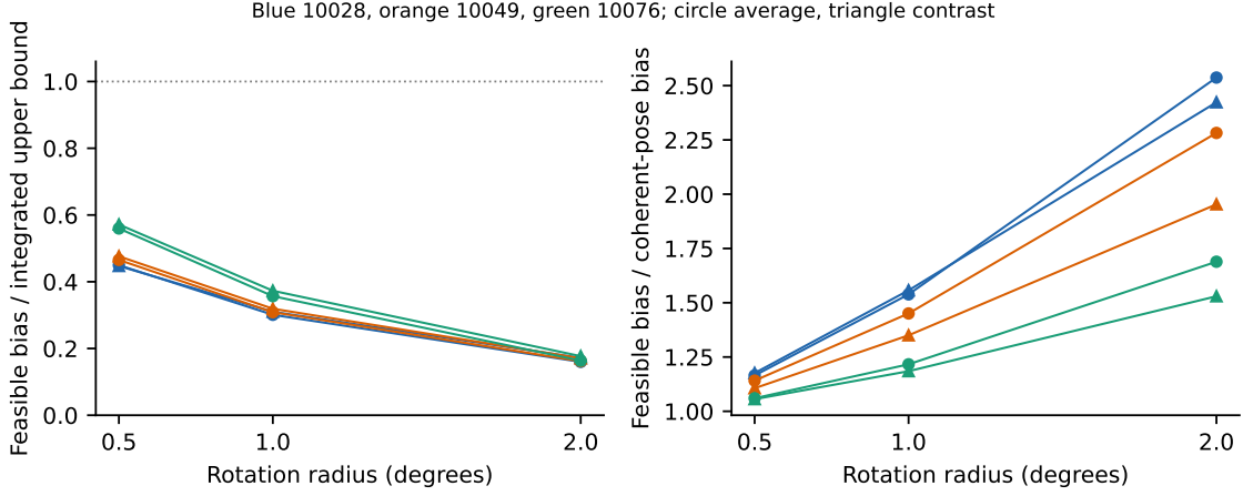
Figure 10. All 18 continuous nonlinear stress settings, retaining the strongest of six feasible searches per setting. The left panel compares numerical feasible bias with the integrated-moment upper bound; the right compares it with the earlier coherent-pose control. Surrogate optimization proposes poses only: final candidates eliminate the full continuous density ball using analytic sinc integrals. The largest independent direct-field relative discrepancy was 5.35 \times 10^{-6} . Remaining upper/lower gaps and local-search limitations preclude a sharpness claim.
