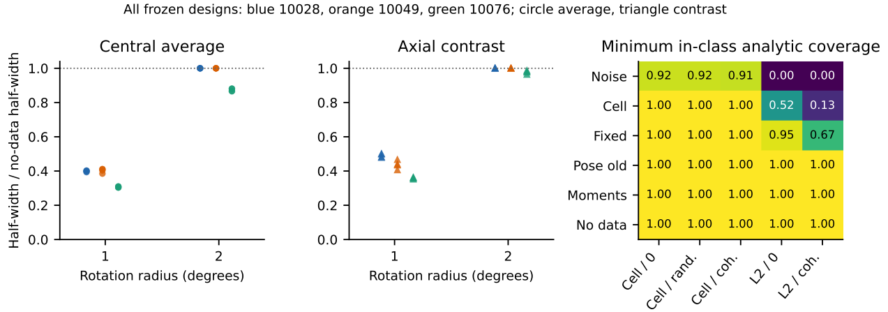
Figure 8. All 48 frozen integrated-moment settings on disjoint particle subsets with new simulation seeds. The original spatial-maximum pose correction falls back to no data throughout; integrated moments retain informative widths in 32 settings. Conservative coverage and poor cell-generator sign power remain limitations. “L2” denotes densities at the declared ball boundary, chosen in the continuous adjoint-residual direction to maximize bias at a fixed pose.
