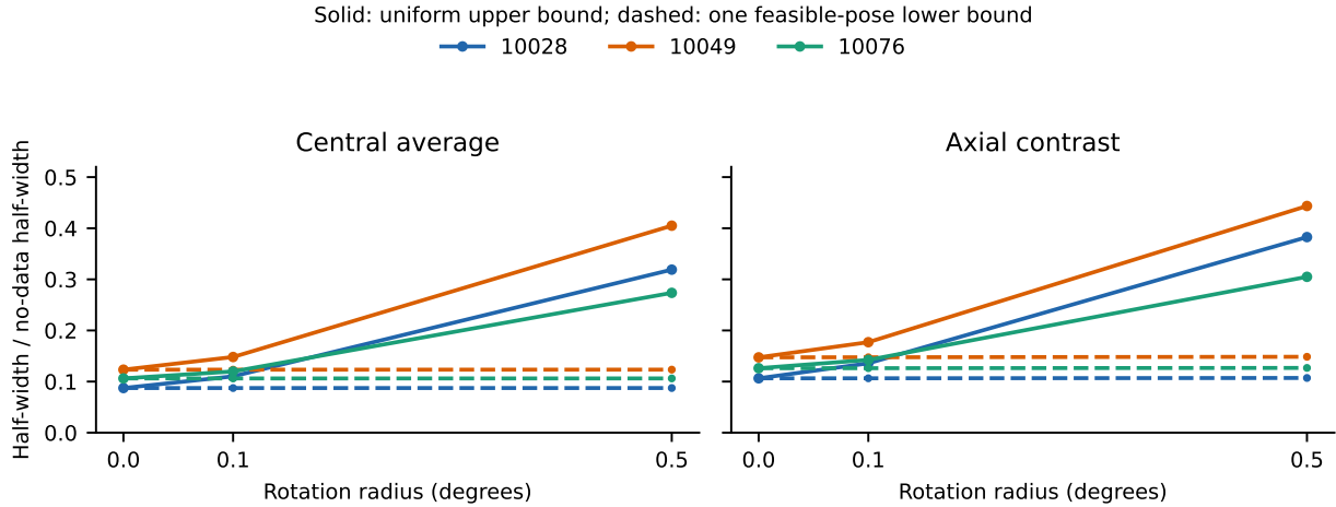
Figure 13. Continuous-density and nonlinear-pose development audit at target width 0.07 of the field. Solid curves are uniform conditional upper bounds for the same fixed-pose-optimized weights. Dashed curves use exact density-ball elimination at one allowed coherent rotation, providing feasible lower bounds on the required width, not global pose optima. Zero is the separate exact-pose control; the nonzero budgets also allow shifts of 0.01/24 field units. The visible gap exposes conservatism.
