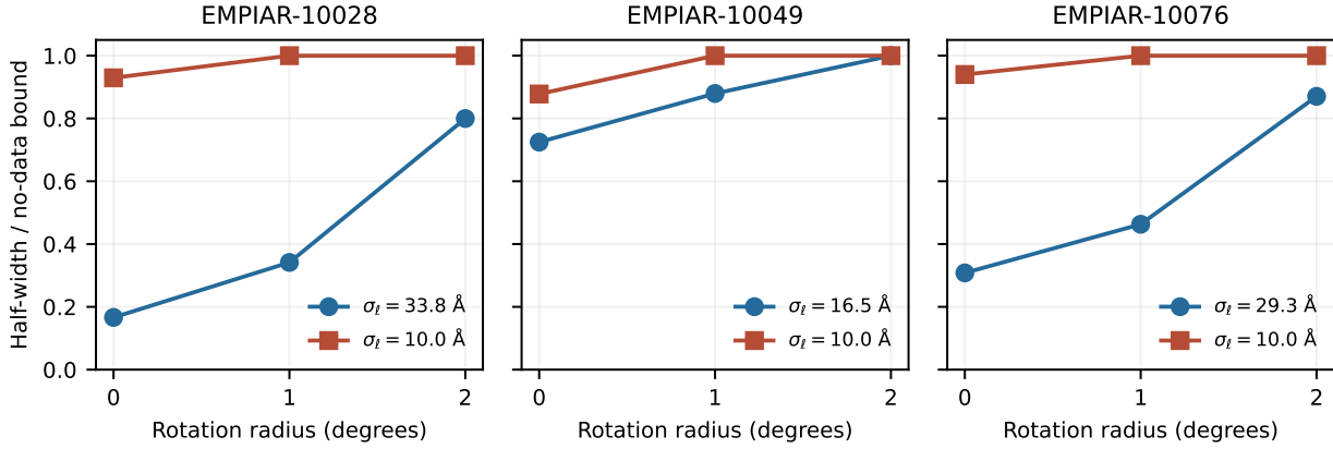
Figure 4. Experimental sensitivity intervals with one inference particle per exposure group. Kernel widths are Gaussian standard deviations, not FSC resolutions. None of these intervals excludes zero. All 10 Å targets switch to the no-data center and width at nonzero pose budgets. Supplied density/pose classes and unverified common-noise/consensus-pose assumptions preclude an experimental coverage claim.
