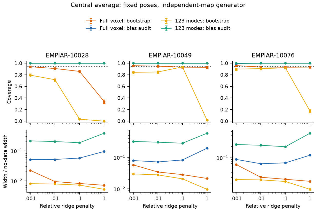
Figure 16. Central-average coverage and widths across all four ridge penalties. Each geometry uses its own fixed independent deposited-map generator. Error bars are binomial 95% intervals over independent measurement-noise draws, conditional on the reused group-bootstrap plan. Weak-regularization bootstrap can be narrow and near nominal; stronger regularization exposes bias. These tests do not establish empirical coverage for unknown experimental density.
