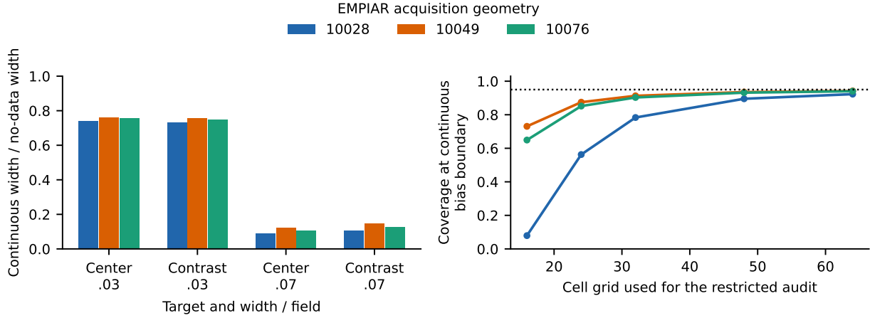
Figure 12. Left: optimized continuous fixed-pose widths for the full cube class. Right: cell-projected audit coverage at a constructed continuous bias boundary, for the broad central target and cell-fitted estimator. Reference-map coverage is one in these cases. The two panels answer distinct questions: useful width and omitted continuous directions.
