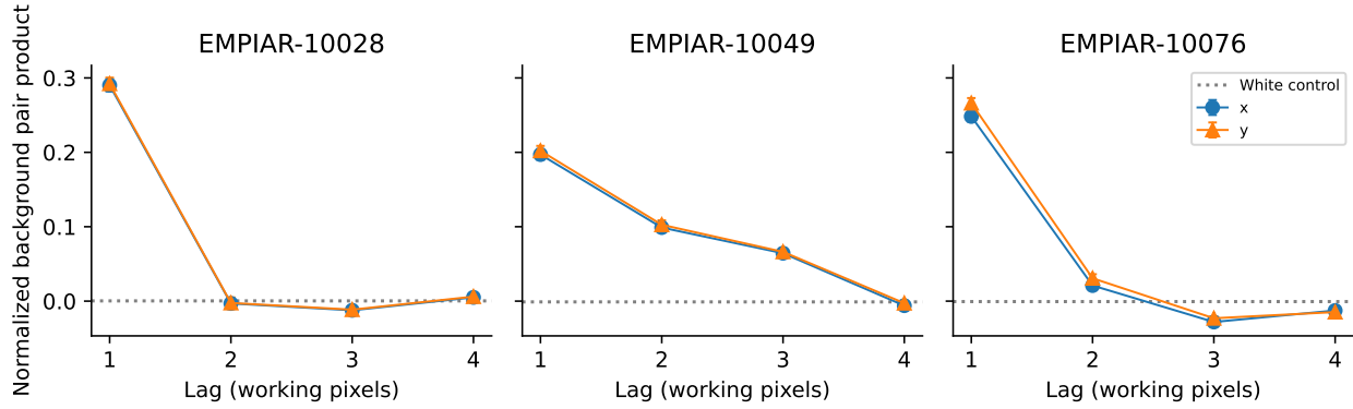
Figure 11. Descriptive background dependence in every additional-exposure image, after Fourier cropping of the downloaded particles to the working grid and before reconstruction windowing. We center and scale each image using pixels outside radius 0.43 of the box, then average products of background pixel pairs separated by each lag. Error bars are marginal 95% whole-exposure bootstrap intervals. Dotted lines show matched-statistic white-Gaussian controls. Background contamination and preprocessing prevent interpreting these values as pure-noise correlations or a confidence calibration.
