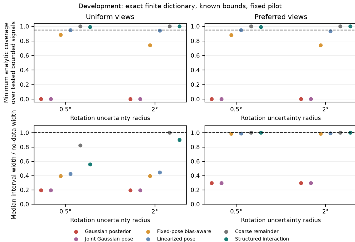
Figure 15. Exact-dictionary development tests with known bounds and an independent fixed pilot. Minimum coverage is over the finite tested set, including adversarial signals; it is not an empirical proof of the worst case. Widths count each independent design once. Gaussian posterior methods separately pass their correctly matched prior-predictive coverage check at 0.95. Their fixed-parameter boundary failures do not contradict Bayesian prior-average calibration.
