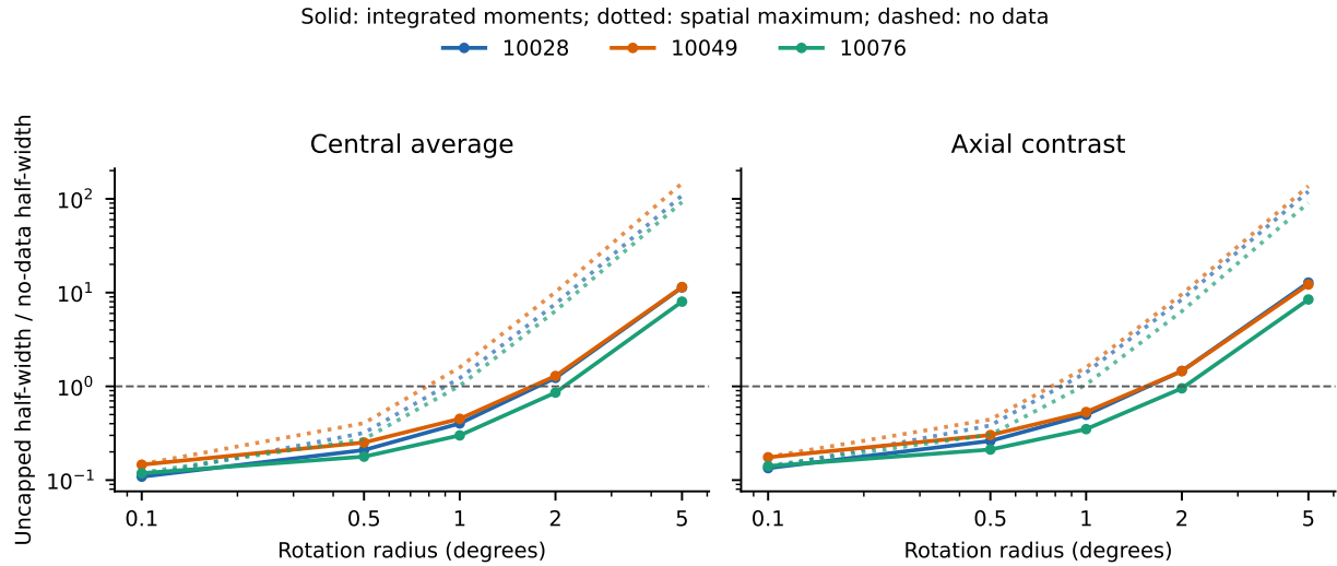
Figure 9. Post-hoc integrated-moment refinement for both broad targets and every tested pose radius. Curves show uncapped widths to expose conservatism; the implemented decision uses the no-data estimator above the dashed line. The solid curves use integrated Fourier-column moments and actual estimator weights; dotted curves use the older spatial-maximum cubic remainder. No weights are refitted.
