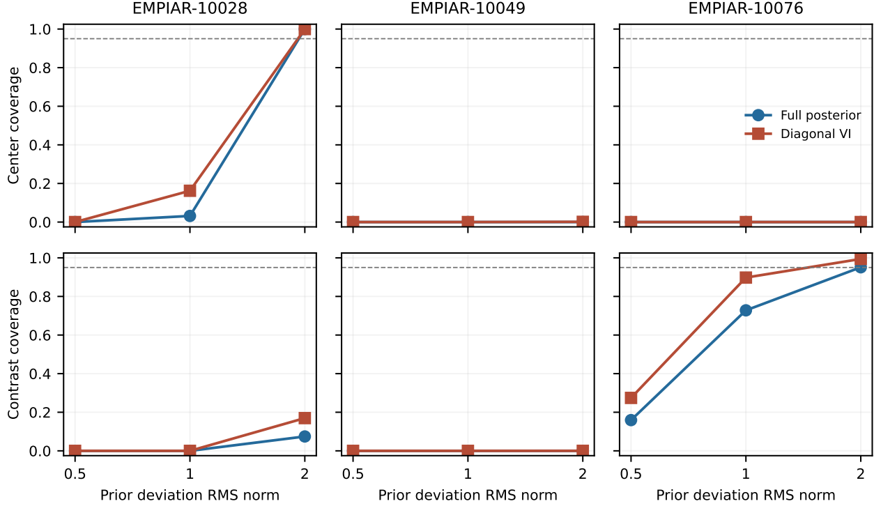
Figure 6. Known-noise coverage for fixed continuous reference densities at nominal poses as the declared Gaussian prior scale varies. The dashed line is 0.95. This is distinct from the full posterior’s matched prior-predictive coverage, which is 0.95 throughout. Diagonal VI is wider here; prior and forward-model discrepancy remain important. No prior scale is selected using these outcomes.
