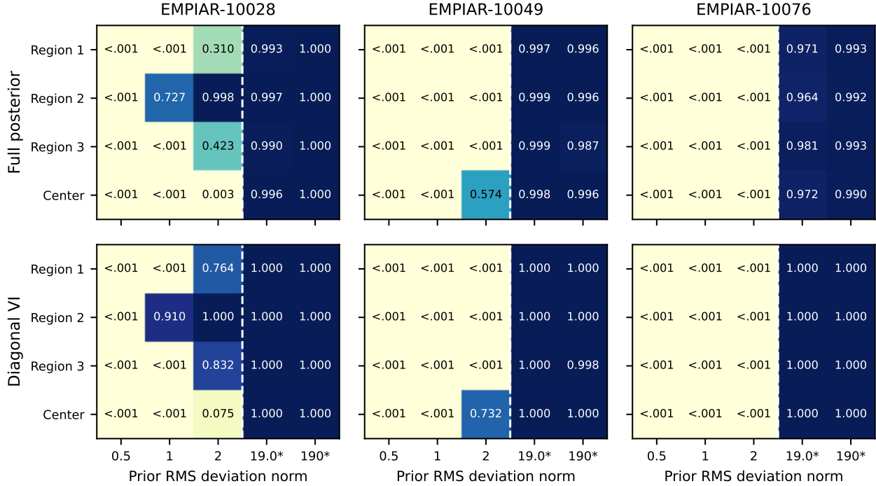
Figure 7. Analytic known-noise pointwise coverage at nominal poses for the four locked targets per stack. Values are rounded; 1.000 need not equal one. The first three columns are the original prior sweep; starred columns are the separately declared broader-prior sensitivity after those outcomes. Full matched prior-predictive coverage is 0.995833 for every prior, whereas these fixed-reference probabilities need not match it. The improving broader priors and wider diagonal intervals are retained without selecting a winner.
