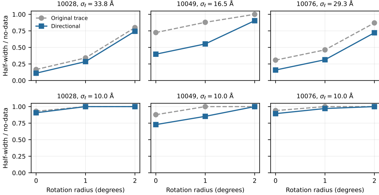
Figure 5. All eighteen experimental directional-noise sensitivity cases. Only the calibration bound changes; weights and continuous bias terms are held fixed. The single interval excluding zero is the broad 10076 target at fixed pose; it does not exclude zero at one degree. Noise, density and pose assumptions remain unverified, and the previously inspected diagnostic pool makes this exploratory reuse rather than a new frozen confirmation.
