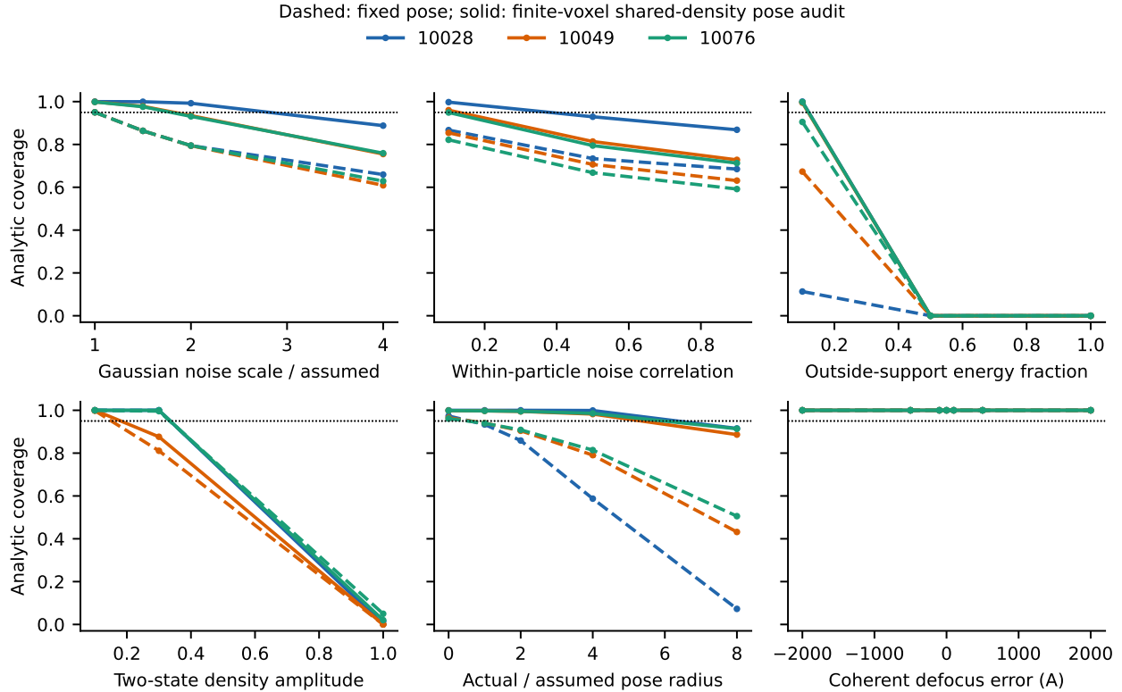
Figure 18. Deliberate assumption stresses for the finite-voxel central target. Curves share a signal within each geometry/control: the fixed-pose boundary for noise tests, a fixed-pose-estimator-directed support or mixture perturbation, or a saved nonlinear pose adversary. Dashed curves are fixed-pose certificates; solid curves include the shared-density pose audit. These are constructed diagnostic conditions, not experimental failure rates. All other controls remain in the result records.
