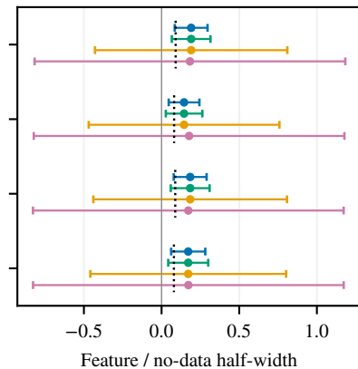
EMPIAR-10076 (heterogeneous)
