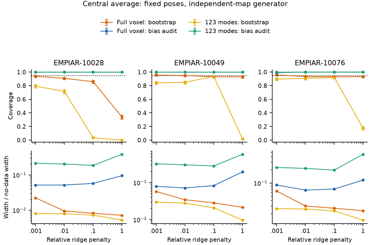
Figure 11. Central-average coverage and widths across all four ridge penalties. Each geometry uses its own fixed independent deposited-map generator. Error bars are binomial 95% intervals over independent measurement-noise draws, conditional on the reused group-bootstrap plan. Weak-regularization bootstrap can be narrow and near nominal; stronger regularization exposes bias. These tests do not establish empirical coverage for unknown experimental density.
