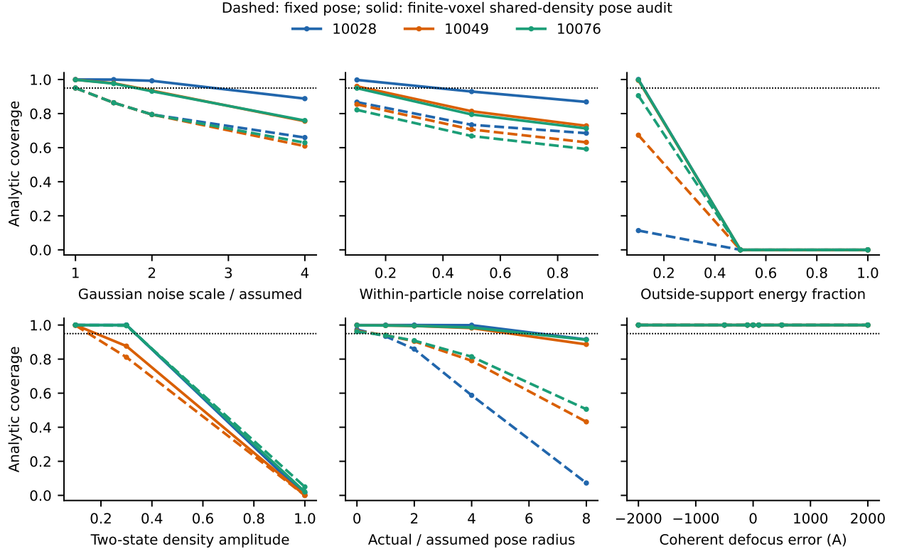
Figure 9. Deliberate assumption stresses for the finite-voxel central target. Curves share a signal within each geometry/control: the fixed-pose boundary for noise tests, a fixed-pose-estimator-directed support or mixture perturbation, or a saved nonlinear pose adversary. Dashed curves are fixed-pose certificates; solid curves include the shared-density pose audit. These are constructed diagnostic conditions, not experimental failure rates. All other controls remain in the result records.
