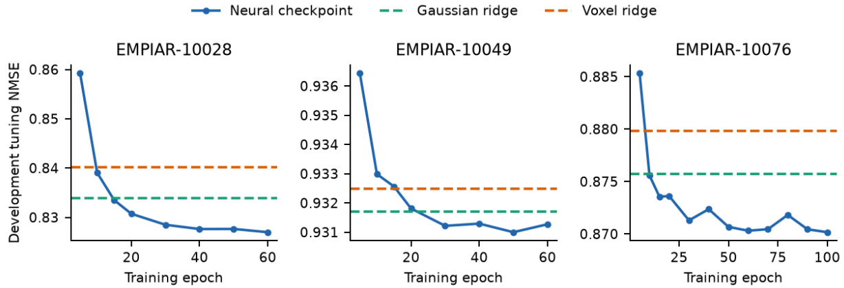
Figure 13. Development tuning error at all evaluated neural checkpoints, with the classical reconstruction controls. Checkpoint selection minimizes this tuning error; the test-group error is not used to select the checkpoint. Different training objectives and supplied consensus poses limit this comparison.
