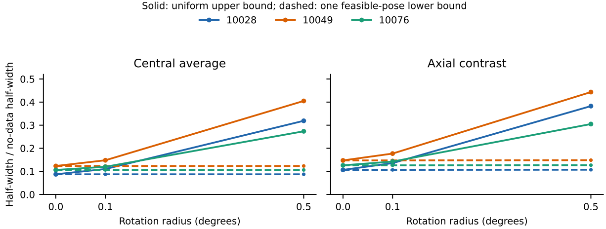
Figure 8. Continuous-density and nonlinear-pose development audit at target width 0.07 of the field. Solid curves are uniform conditional upper bounds for the same fixed-pose-optimized weights. Dashed curves use exact density-ball elimination at one allowed coherent rotation, providing feasible lower bounds on the required width, not global pose optima. Zero is the separate exact-pose control; the nonzero budgets also allow shifts of 0.01/24 field units. The visible gap exposes conservatism.
