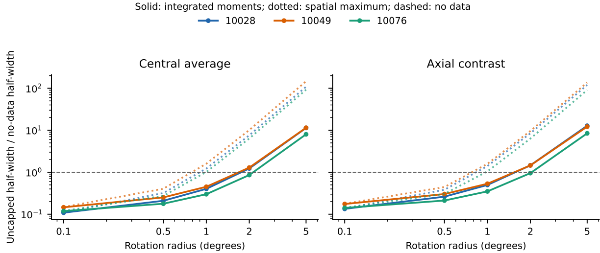
Figure 4. Post-hoc integrated-moment refinement for both broad targets and every tested pose radius. Curves show uncapped widths to expose conservatism; the implemented decision uses the no-data estimator above the dashed line. The solid curves use integrated Fourier-column moments and actual estimator weights; dotted curves use the older spatial-maximum cubic remainder. No weights are refitted.
