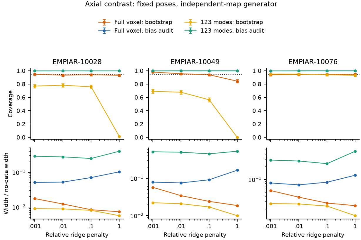
Figure 12. The same complete regularization comparison for the axial contrast. Both the estimand and the unknown simulation signal are fixed before noise replication. The full results also retain the smaller 33-mode dictionary, basic bootstrap and Gaussian covariance controls.
