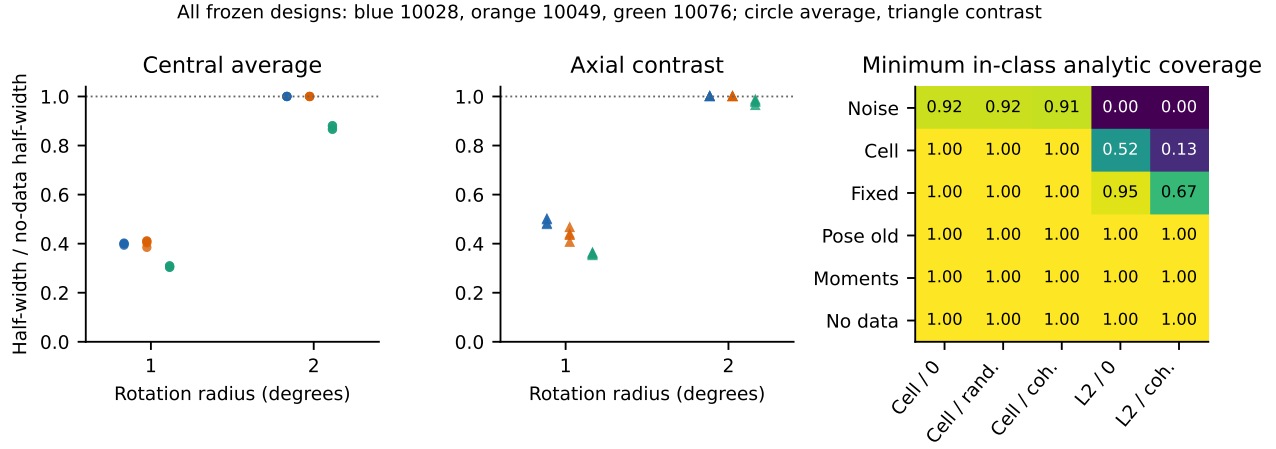
Figure 3. All 48 frozen integrated-moment settings on disjoint particle subsets with new simulation seeds. The original spatial-maximum pose correction falls back to no data throughout; integrated moments retain informative widths in 32 settings. Conservative coverage and poor cell-generator sign power remain limitations. “L2” denotes constructed continuous-density boundaries.
