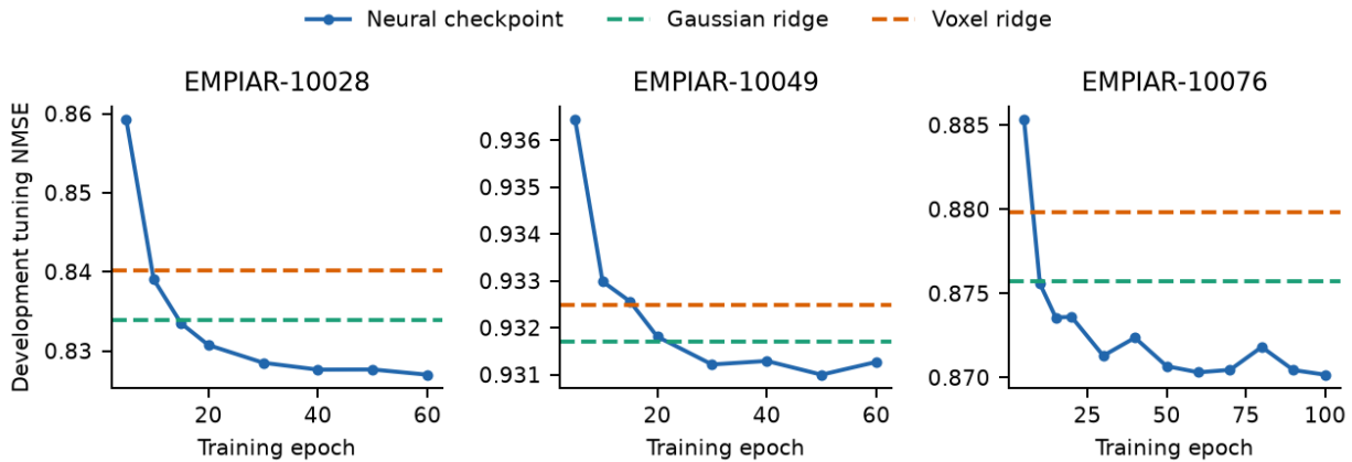
Figure 19. Development tuning error at all evaluated neural checkpoints, with the classical reconstruction controls. Checkpoint selection minimizes this tuning error; the test-group error is not used to select the checkpoint. Different training objectives and supplied consensus poses limit this comparison.
