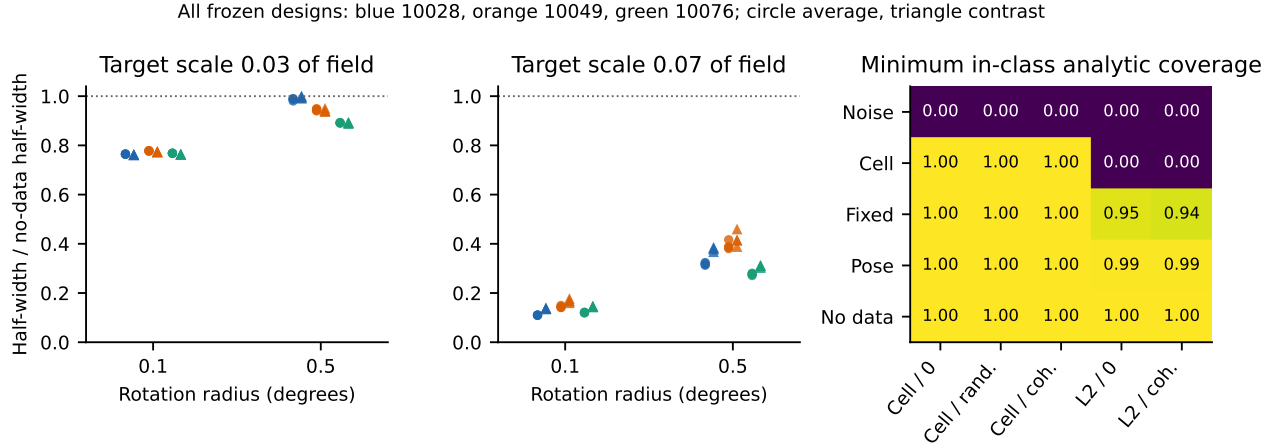
Figure 2. Completed frozen original-audit study: all 96 settings. Each geometry contributes both feature targets at each scale and pose budget. Width is relative to the same density class’s no-data interval. The right panel reports minimum analytic coverage by generator/scenario group; “L2” denotes densities at the declared ball boundary, chosen in the continuous adjoint-residual direction to maximize bias at a fixed pose. Values are rounded for display. Fine-feature widths near one and conservative cell-generator coverage limit a usefulness interpretation.
