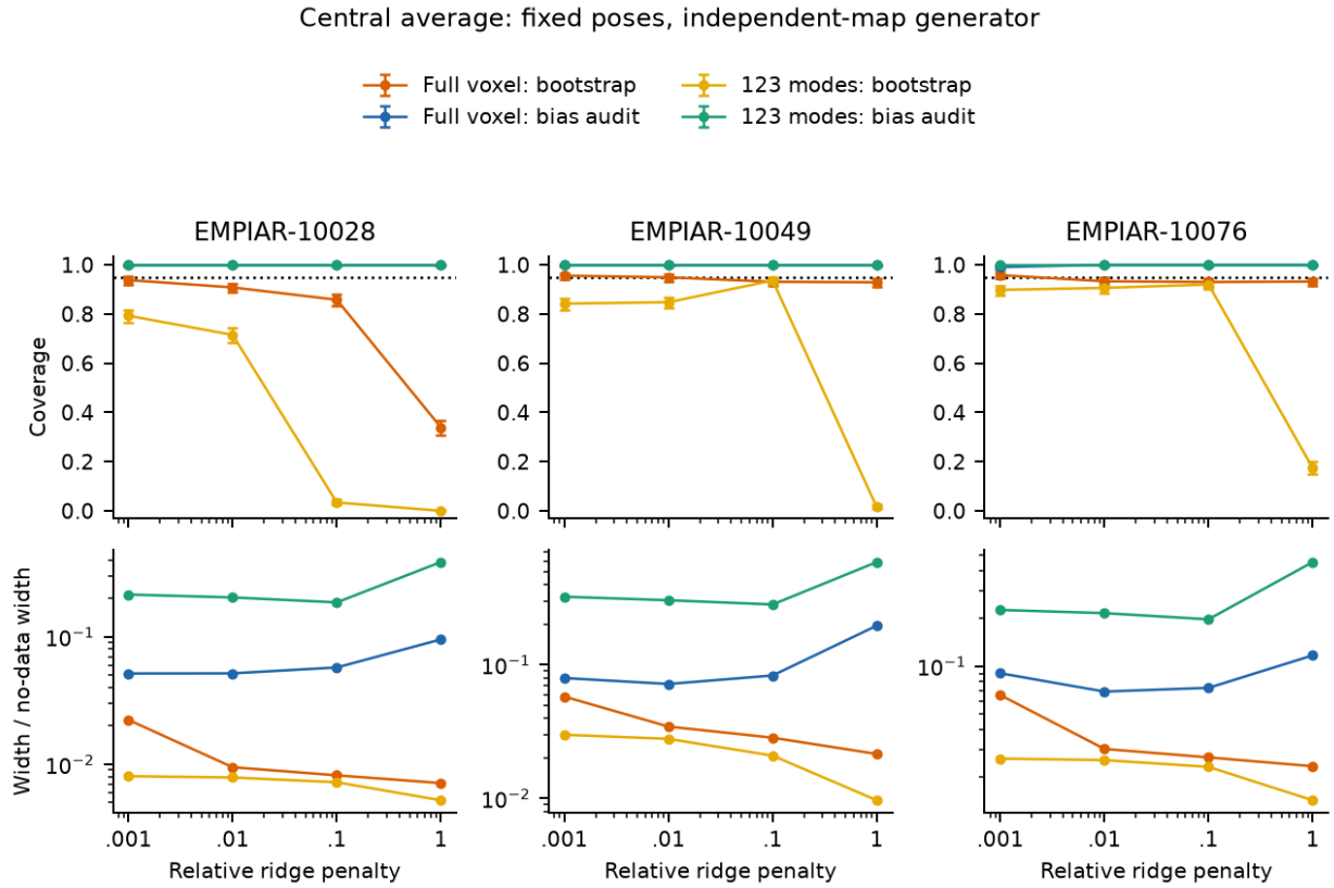
Figure 17. Central-average coverage and widths across all four ridge penalties. Each geometry uses its own fixed independent deposited-map generator. Error bars are binomial 95% intervals over independent measurement-noise draws, conditional on the reused group-bootstrap plan. Weak-regularization bootstrap can be narrow and near nominal; stronger regularization exposes bias. These tests do not establish empirical coverage for unknown experimental density.
