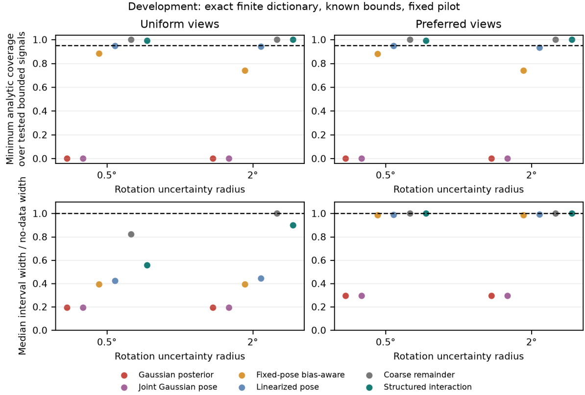
Figure 8. Exact-dictionary development tests with known bounds and an independent fixed pilot. Minimum coverage is over the finite tested set, including adversarial signals; it is not an empirical proof of the worst case. Widths count each independent design once. Gaussian posterior methods separately pass their correctly matched prior-predictive coverage check at 0.95. Their fixed-parameter boundary failures do not contradict Bayesian prior-average calibration.
