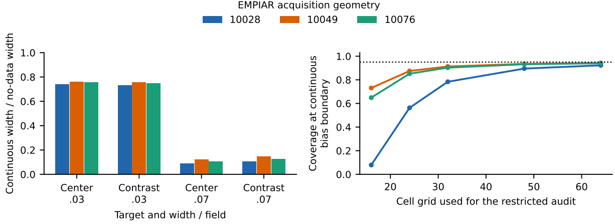
Figure 5. Left: optimized continuous fixed-pose widths for the full cube class. Right: cell-projected audit coverage at a constructed continuous bias boundary, for the broad central target and cell-fitted estimator. Reference-map coverage is one in these cases. The two panels answer distinct questions: useful width and omitted continuous directions.
