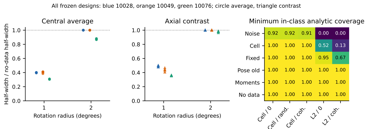
Figure 14. All 48 frozen integrated-moment settings on disjoint particle subsets with new simulation seeds. The original spatial-maximum pose correction falls back to no data throughout; integrated moments retain informative widths in 32 settings. Conservative coverage and poor cell-generator sign power remain limitations. “L2” denotes densities at the declared ball boundary, chosen in the continuous adjoint-residual direction to maximize bias at a fixed pose.
