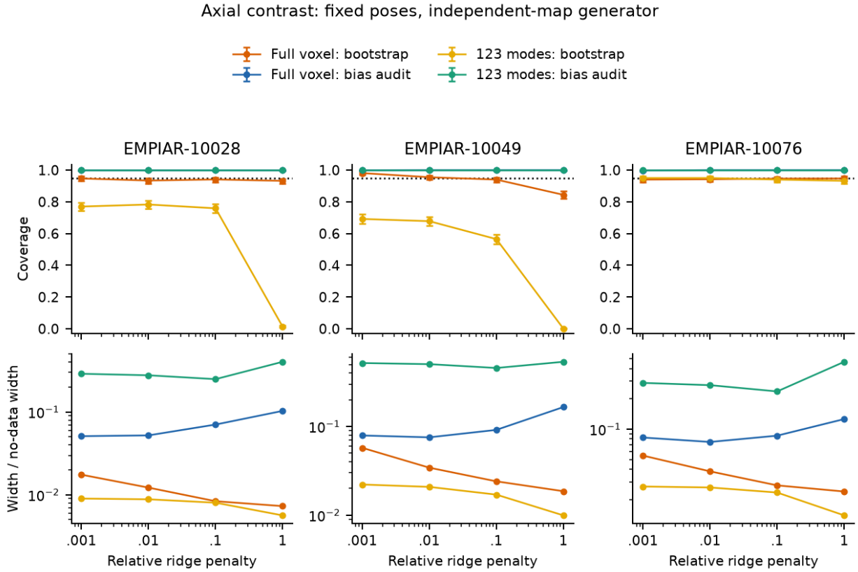
Figure 23. The same complete regularization comparison for the axial contrast. Both the estimand and the unknown simulation signal are fixed before noise replication. The full results also retain the smaller 33-mode dictionary, basic bootstrap and Gaussian covariance controls.
