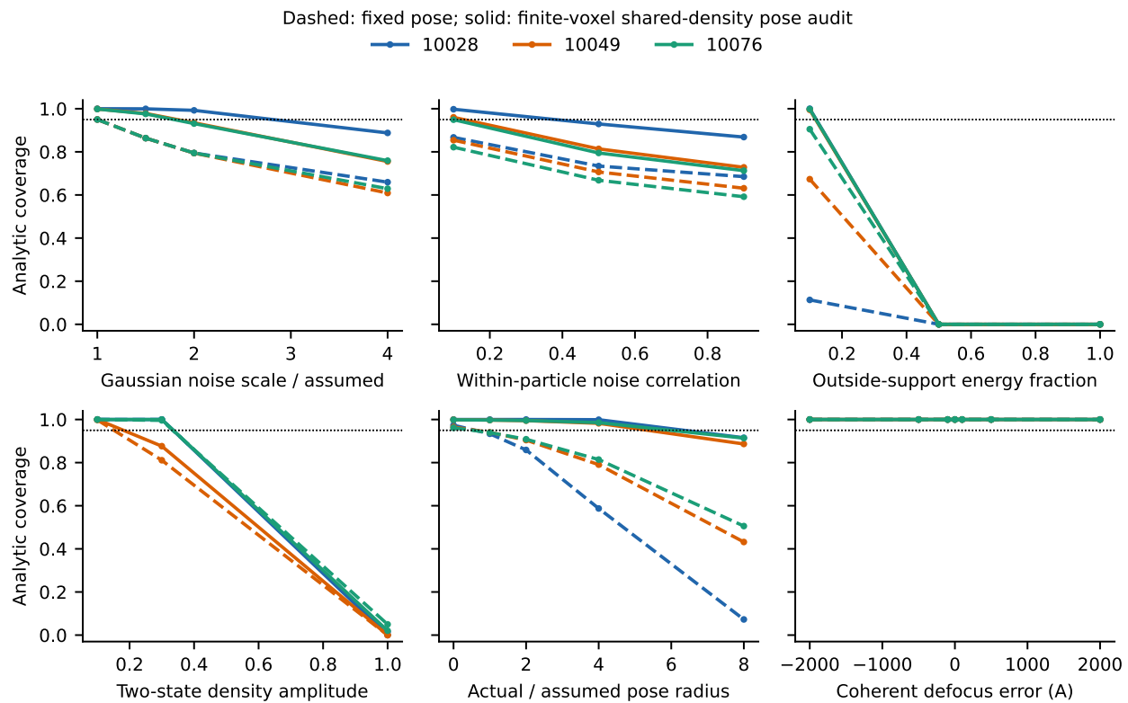
Figure 20. Deliberate assumption stresses for the finite-voxel central target. Curves share a signal within each geometry/control: the fixed-pose boundary for noise tests, a fixed-pose-estimator-directed support or mixture perturbation, or a saved nonlinear pose adversary. Dashed curves are fixed-pose certificates; solid curves include the shared-density pose audit. These are constructed diagnostic conditions, not experimental failure rates. All other controls remain in the result records.
