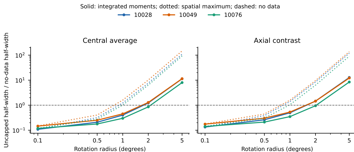
Figure 15. Post-hoc integrated-moment refinement for both broad targets and every tested pose radius. Curves show uncapped widths to expose conservatism; the implemented decision uses the no-data estimator above the dashed line. The solid curves use integrated Fourier-column moments and actual estimator weights; dotted curves use the older spatial-maximum cubic remainder. No weights are refitted.
