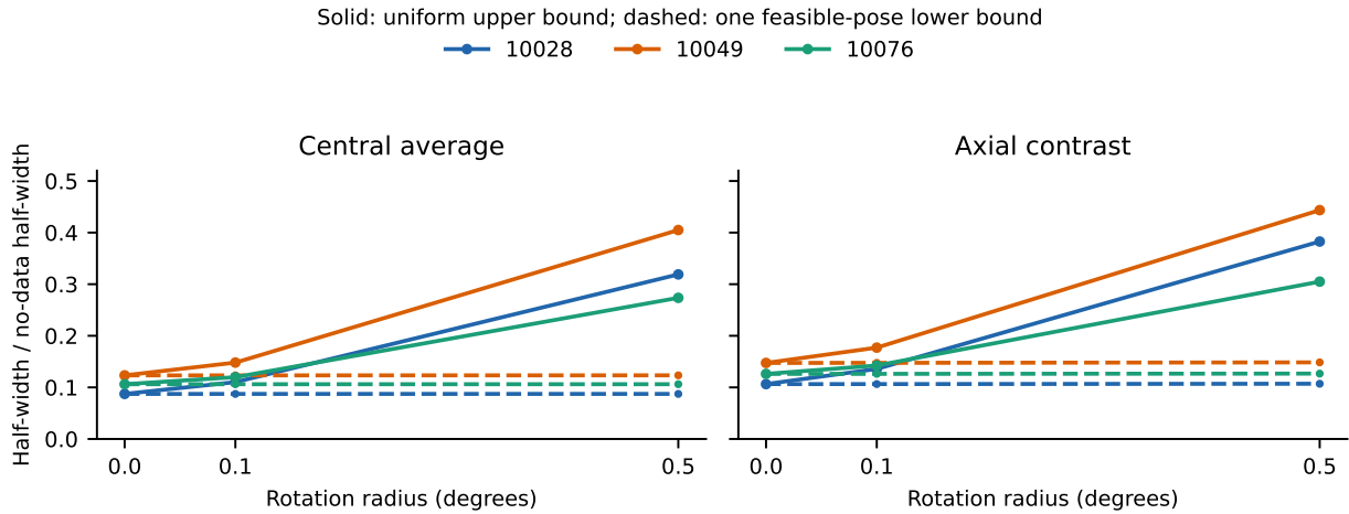
Figure 19. Continuous-density and nonlinear-pose development audit at target width 0.07 of the field. Solid curves are uniform conditional upper bounds for the same fixed-pose-optimized weights. Dashed curves use exact density-ball elimination at one allowed coherent rotation, providing feasible lower bounds on the required width, not global pose optima. Zero is the separate exact-pose control; the nonzero budgets also allow shifts of 0.01/24 field units. The visible gap exposes conservatism.
