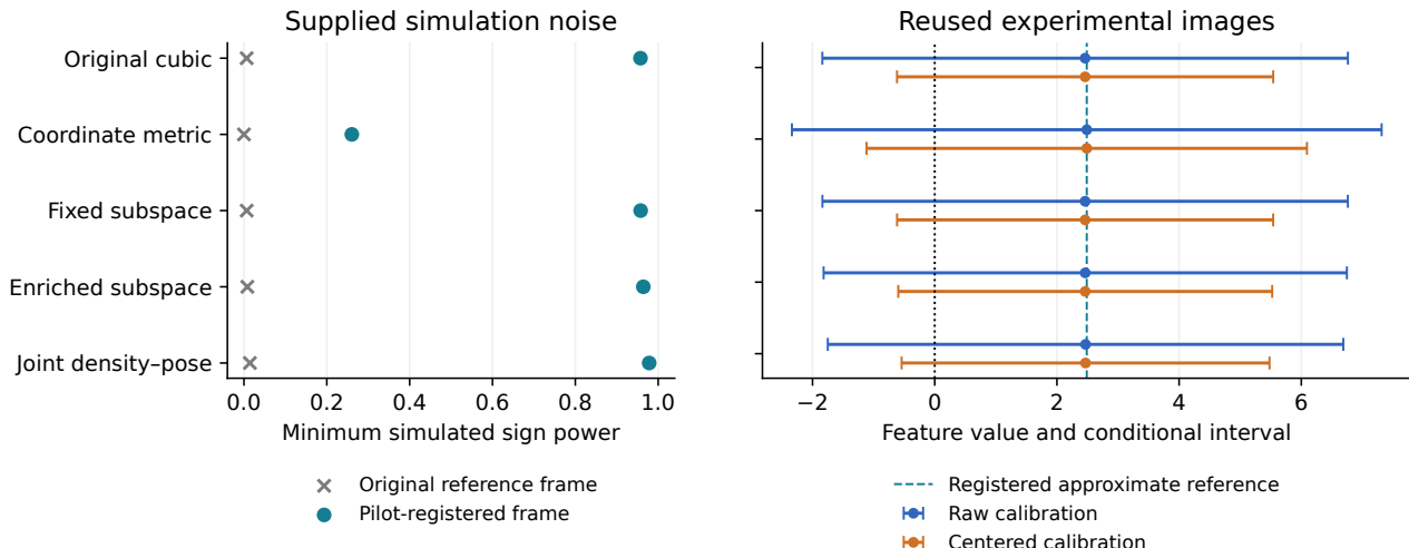
Figure 12. All five cubic designs on the selected 10049 region. Left: minimum conditional simulated sign power across three declared poses, retaining both reference frames. Right: observed intervals under separately reported raw and centered calibration; all contain zero. Each procedure retains the stated .05/12 total error allocation under unverified model premises; the plot is not an experimental coverage claim or an unadjusted selection rule across procedures. The registered approximate reference is not biological truth.
