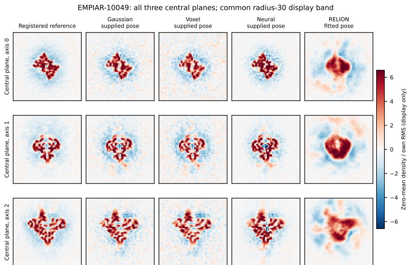
Figure 6. EMPIAR-10049: all three central planes of the registered reference and four existing reconstructions. Each square spans 236.16 \text{ \AA} . The display removes DC, retains a common radius-30 Fourier band, and divides each map by its own volumetric RMS; a pooled 99.5th-percentile absolute value fixes the common symmetric color range. This display normalization hides amplitude differences and is not used for FSC or intervals. Views are fixed array planes, not selected for agreement. Gaussian, voxel and neural estimates average the locked halves; RELION uses its previously evaluated map. Registration is pilot-derived. The 10076 reference represents Class A, not the heterogeneous consensus.
