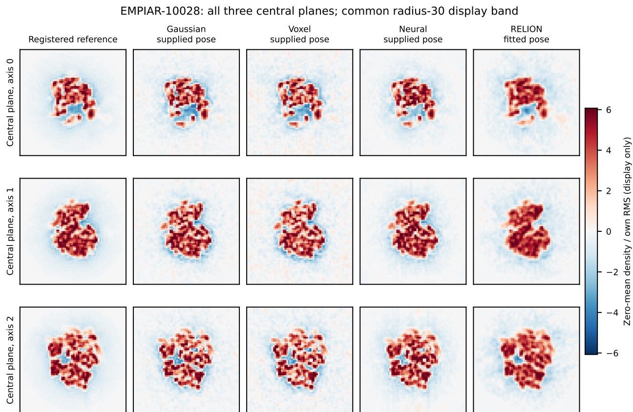
Figure 5. EMPIAR-10028: all three central planes of the registered reference and four existing reconstructions. Each square spans 482.4 \text{ \AA} . The display removes DC, retains a common radius-30 Fourier band, and divides each map by its own volumetric RMS; a pooled 99.5th-percentile absolute value fixes the common symmetric color range. This display normalization hides amplitude differences and is not used for FSC or intervals. Views are fixed array planes, not selected for agreement. Gaussian, voxel and neural estimates average the locked halves; RELION uses its previously evaluated map. Registration is pilot-derived. The 10076 reference represents Class A, not the heterogeneous consensus.
