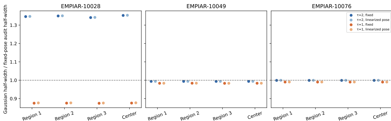
Figure 3. All twelve locked features and four continuous Gaussian comparisons. The dashed line denotes the original fixed-pose audit width. Matched prior scale \tau = 2 gives near-equal widths on two stacks; its 10028 widths are 34–35% larger. The half-scale prior is narrower without the same uniform class implication. Adding the specified first-order Gaussian pose covariance has little effect here. Every fit converged.
