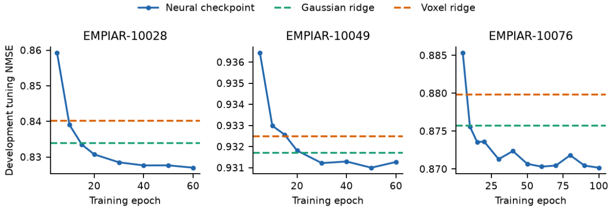
Figure 15. Development tuning error at all evaluated neural checkpoints, with the classical reconstruction controls. Checkpoint selection minimizes this tuning error; the test-group error is not used to select the checkpoint. Different training objectives and supplied consensus poses limit this comparison.
