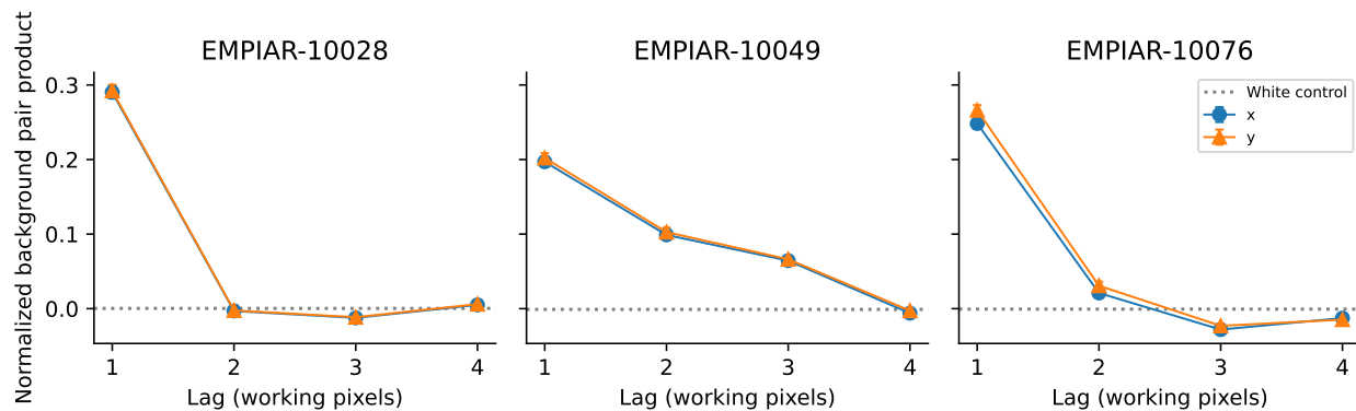
Figure 8. Descriptive background dependence in every additional-exposure image, after Fourier cropping of the downloaded particles to the working grid and before reconstruction windowing. We center and scale each image using pixels outside radius 0.43 of the box, then average products of background pixel pairs separated by each lag. Error bars are marginal 95% whole-exposure bootstrap intervals. Dotted lines show matched-statistic white-Gaussian controls. Background contamination and preprocessing prevent interpreting these values as pure-noise correlations or a confidence calibration.
