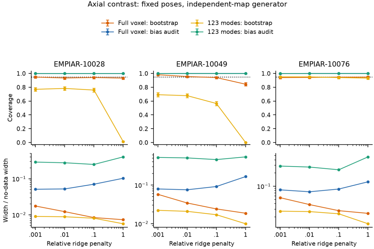
Figure 14. The same complete regularization comparison for the axial contrast. Both the estimand and the unknown simulation signal are fixed before noise replication. The full results also retain the smaller 33-mode dictionary, basic bootstrap and Gaussian covariance controls.
