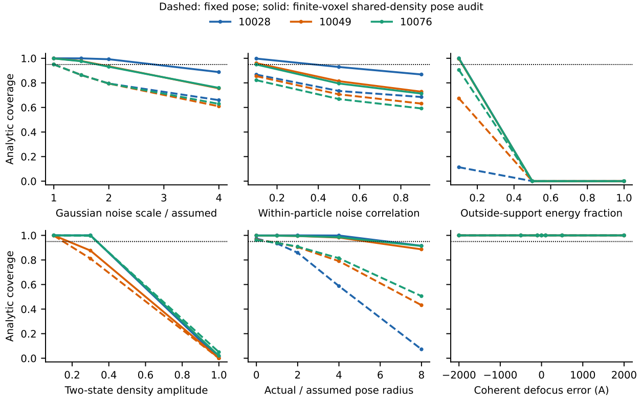
Figure 11. Deliberate assumption stresses for the finite-voxel central target. Curves share a signal within each geometry/control: the fixed-pose boundary for noise tests, a fixed-pose-estimator-directed support or mixture perturbation, or a saved nonlinear pose adversary. Dashed curves are fixed-pose certificates; solid curves include the shared-density pose audit. These are constructed diagnostic conditions, not experimental failure rates. All other controls remain in the result records.
