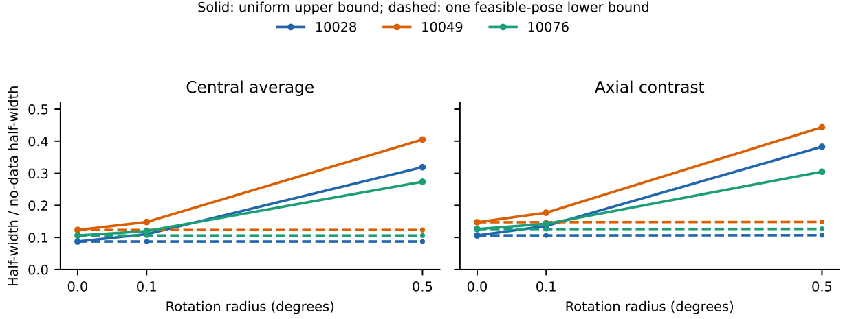
Figure 10. Continuous-density and nonlinear-pose development audit at target width 0.07 of the field. Solid curves are uniform conditional upper bounds for the same fixed-pose-optimized weights. Dashed curves use exact density-ball elimination at one allowed coherent rotation, providing feasible lower bounds on the required width, not global pose optima. Zero is the separate exact-pose control; the nonzero budgets also allow shifts of 0.01/24 field units. The visible gap exposes conservatism.
