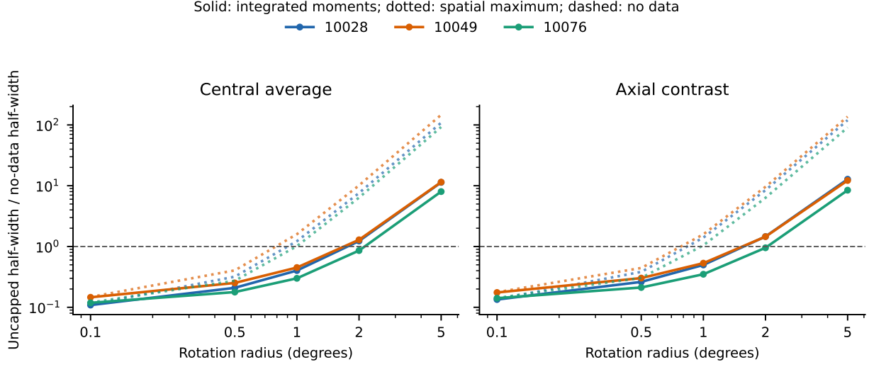
Figure 6. Post-hoc integrated-moment refinement for both broad targets and every tested pose radius. Curves show uncapped widths to expose conservatism; the implemented decision uses the no-data estimator above the dashed line. The solid curves use integrated Fourier-column moments and actual estimator weights; dotted curves use the older spatial-maximum cubic remainder. No weights are refitted.
