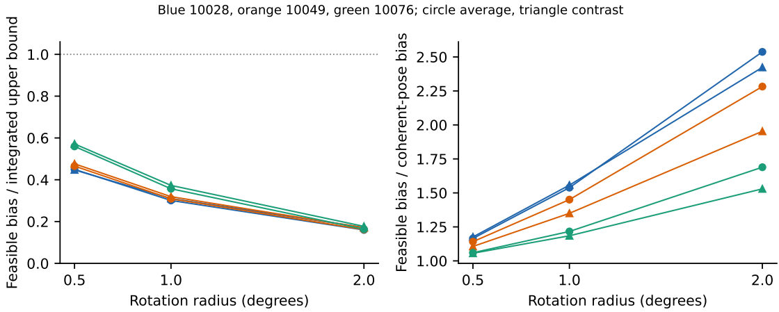
Figure 7. All 18 continuous nonlinear stress settings, retaining the strongest of six feasible searches per setting. The left panel compares numerical feasible bias with the integrated-moment upper bound; the right compares it with the earlier coherent-pose control. Surrogate optimization proposes poses only: final candidates eliminate the full continuous density ball using analytic sinc integrals. The largest independent direct-field relative discrepancy was 5.35 \times 10^{-6} . Remaining upper/lower gaps and local-search limitations preclude a sharpness claim.
