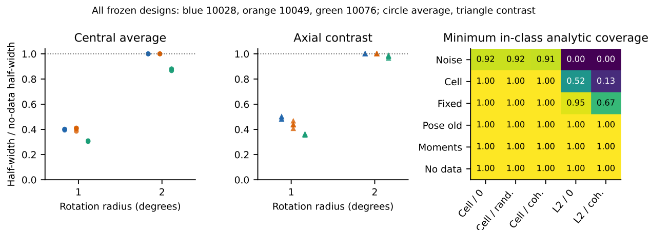
Figure 5. All 48 frozen integrated-moment settings on disjoint particle subsets with new simulation seeds. The original spatial-maximum pose correction falls back to no data throughout; integrated moments retain informative widths in 32 settings. Conservative coverage and poor cell-generator sign power remain limitations. “L2” denotes densities at the declared ball boundary, chosen in the continuous adjoint-residual direction to maximize bias at a fixed pose.
