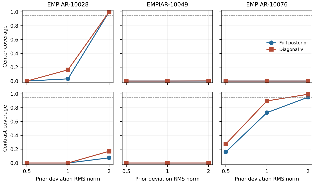
Figure 4. Known-noise coverage for fixed continuous reference densities at nominal poses as the declared Gaussian prior scale varies. The dashed line is 0.95. This is distinct from the full posterior’s matched prior-predictive coverage, which is 0.95 throughout. Diagonal VI is wider here; prior and forward-model discrepancy remain important. No prior scale is selected using these outcomes.
