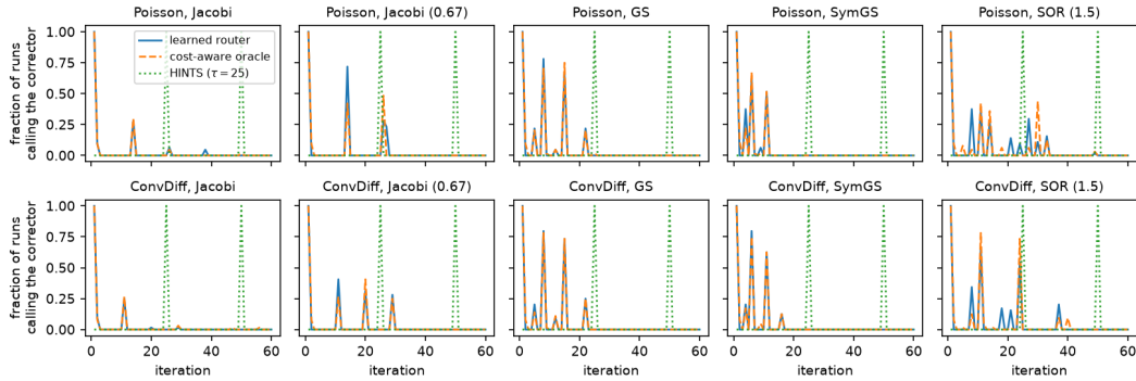
Figure 13: Corrector usage: fraction of test runs that execute a corrector call at each iteration, for the learned router, the cost-aware oracle and HINTS ( \tau = 25 ). The router calls the corrector once at the start, spends a solver-dependent number of sweeps on the high-frequency band, and calls it again only when the smooth error has re-emerged; HINTS waits 24 sweeps before its first call.
