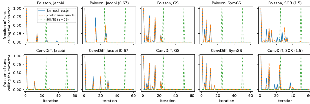
Figure 3: Corrector usage on the 128 \times 128 grid: fraction of test runs that execute a corrector call at each iteration, for the learned router, the cost-aware oracle and HINTS ( \tau=25 ), for every solver pairing (columns) and both equations (rows).
