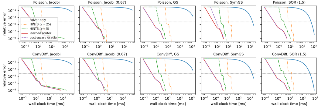
Figure 15: Relative error against charged wall-clock time for one test instance per pairing. The dashed horizontal line is \varepsilon = h^2 .
