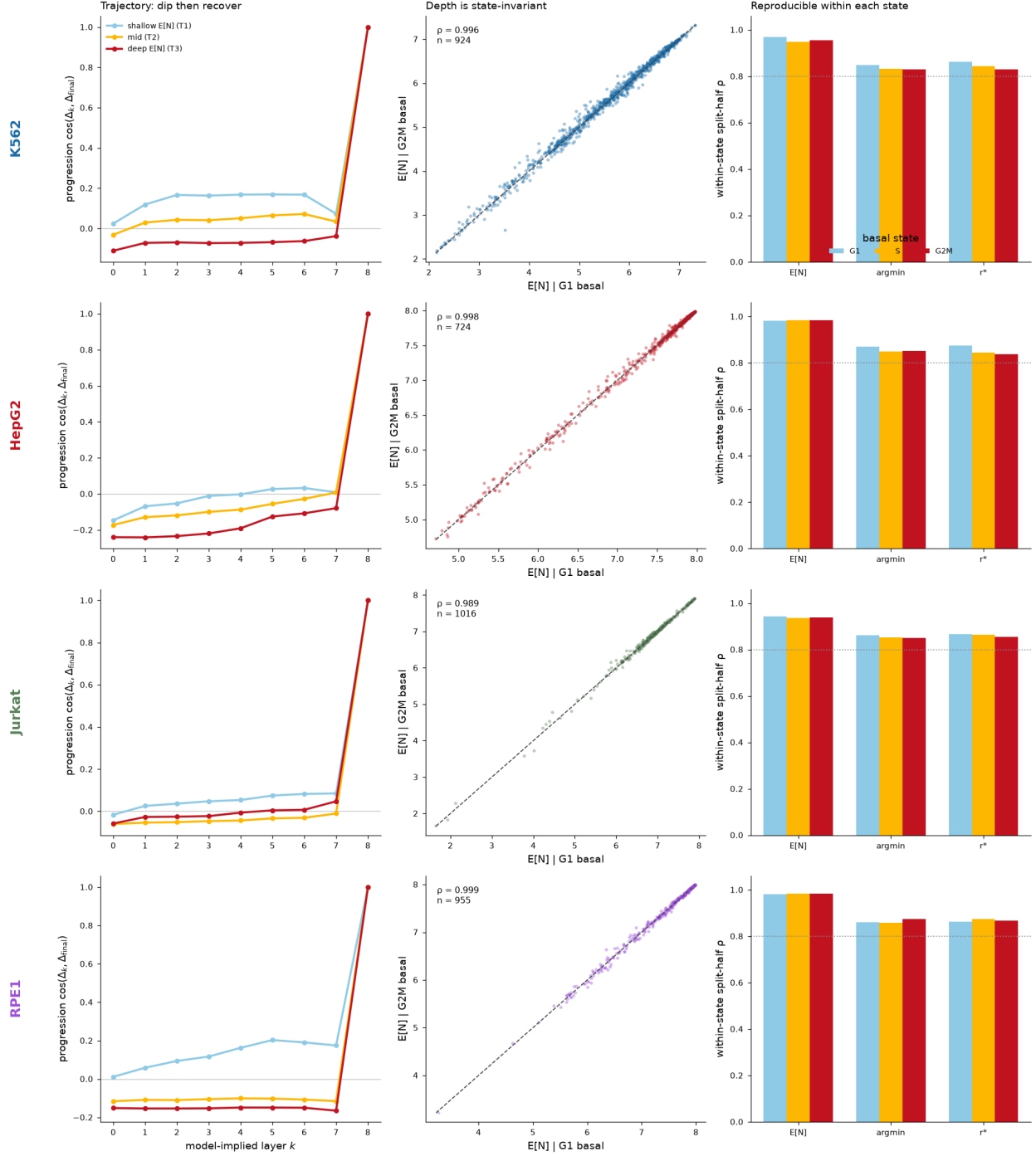
Figure 12: Cell-state robustness of refinement depth (exploratory, four frozen Replogle lines, each analysed on its own data). Rows: K562, HepG2, Jurkat, RPE1. Left: model-implied trajectory — deep- \mathbb{E}[N] perturbations (red) dip mid-trajectory then recover; shallow (blue) approach monotonically. Middle: \mathbb{E}[N] conditioned on G1 vs G2M basal state lies on the diagonal ( \rho = 0.996\text{--}0.999 ): depth is state-invariant. Right: within-state split-half reproducibility of \mathbb{E}[N] /argmin/ r^* ( \rho \geq 0.83 in every state and line). Halting is read from the frozen backbones with no retraining and no temporal labels.
