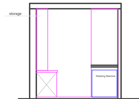
ELEVATION CC
