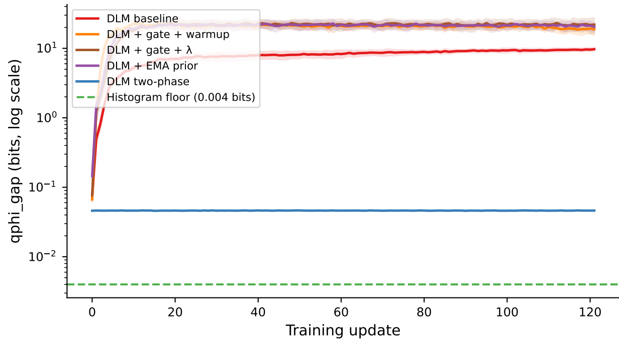
(B) Log scale: gap starts low then explodes (B1-B3 make it worse)
