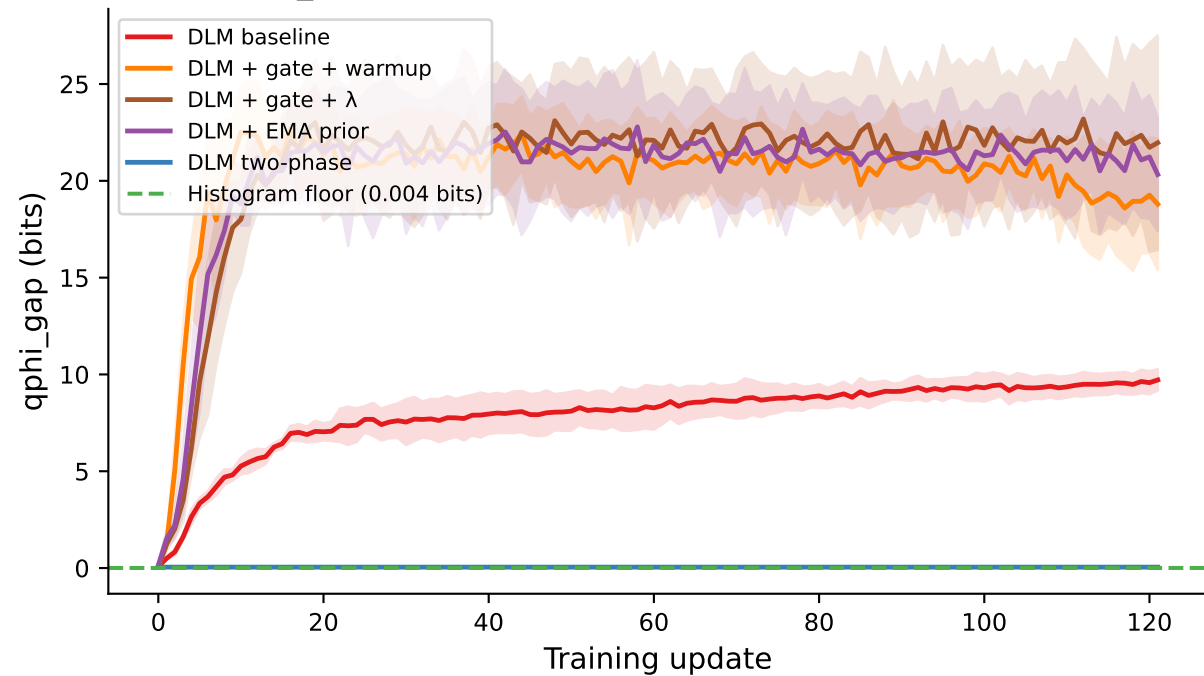
(A) qphi_gap vs training: circular gradient drives gap upward
