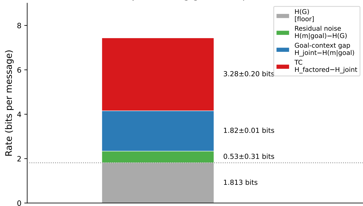
(B) Gap attribution: what each context level saves (TC = joint coding gain, free post-hoc)
