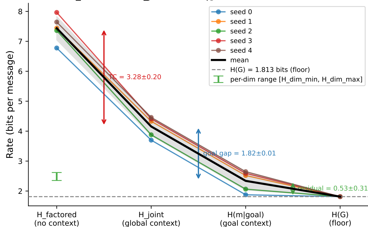
(A) Bound ordering holds for all 5 seeds H_{\text{factored}} \geq H_{\text{joint}} \geq H(m|\text{goal}) \geq H(G) [OK=True]
