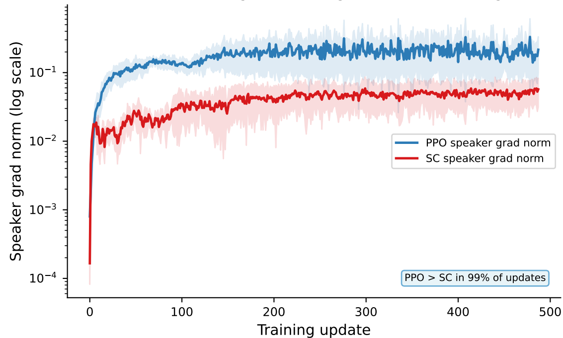
(A) PPO vs SC gradient magnitude over training
