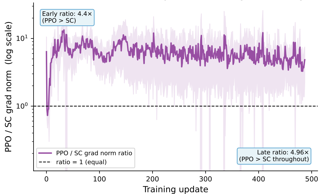
(B) Ratio: PPO consistently leads SC throughout training
