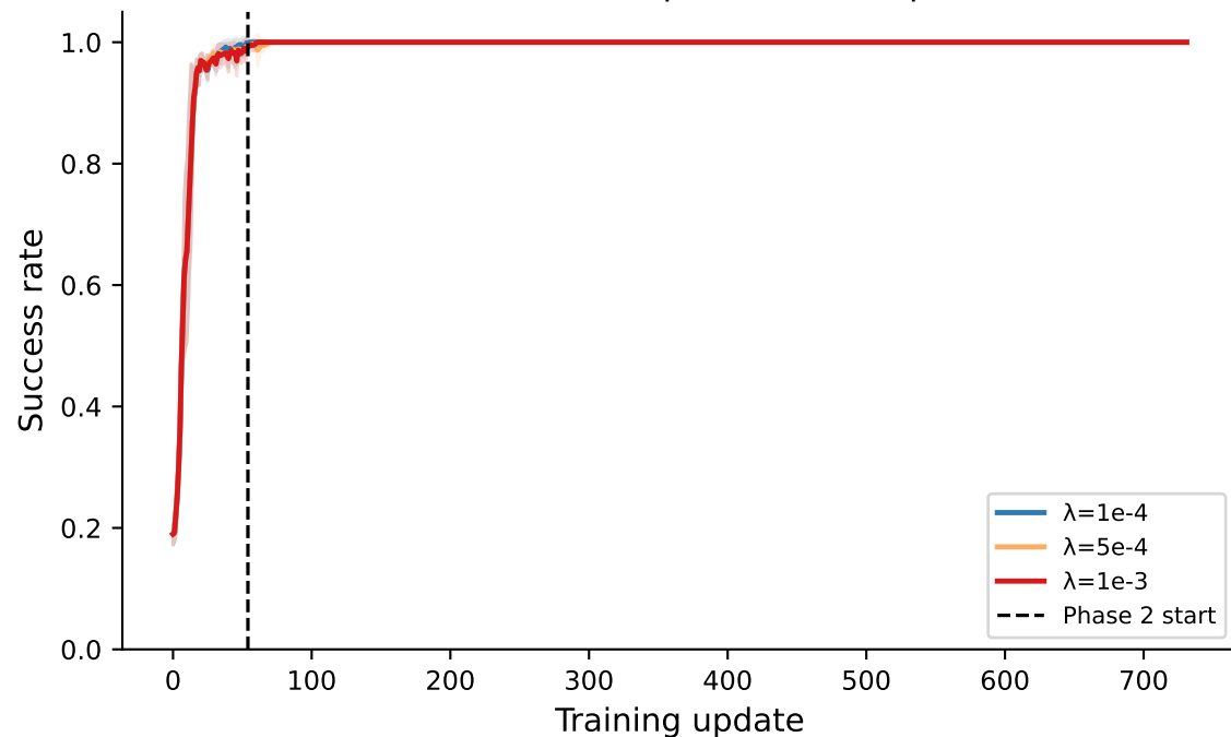
(B) SR maintained \geq 0.98 throughout Phase 2 (E39 listener fix prevents collapse)
