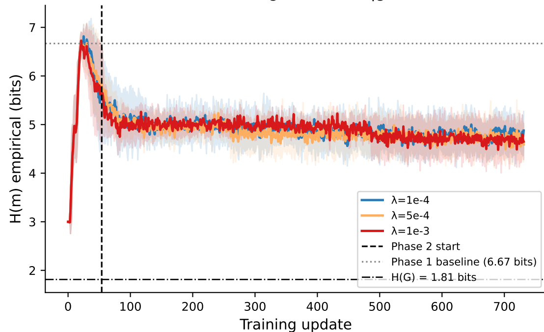
(A) H(m) decreases after Phase 2 triggers (corrected dither loss: genuine H(m|goal) reduction)
