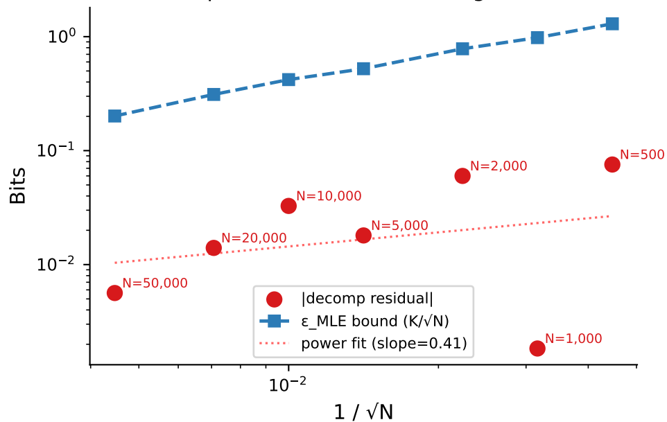
(A) Decomposition residual converges as O(1/\sqrt{N})
