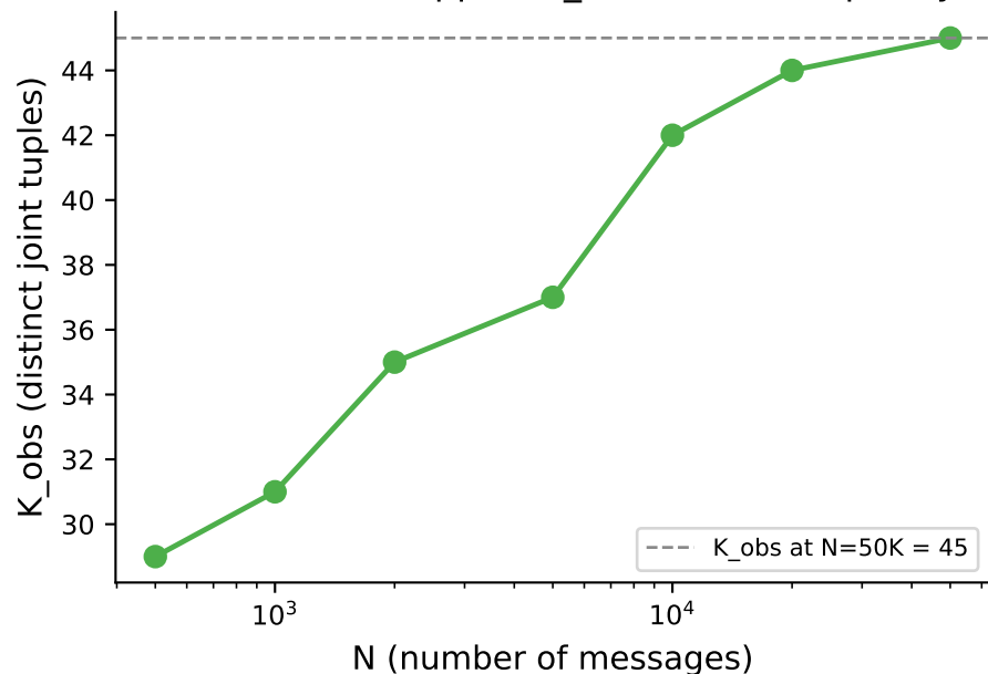
(B) Observed support K_{\text{obs}} stabilises quickly
