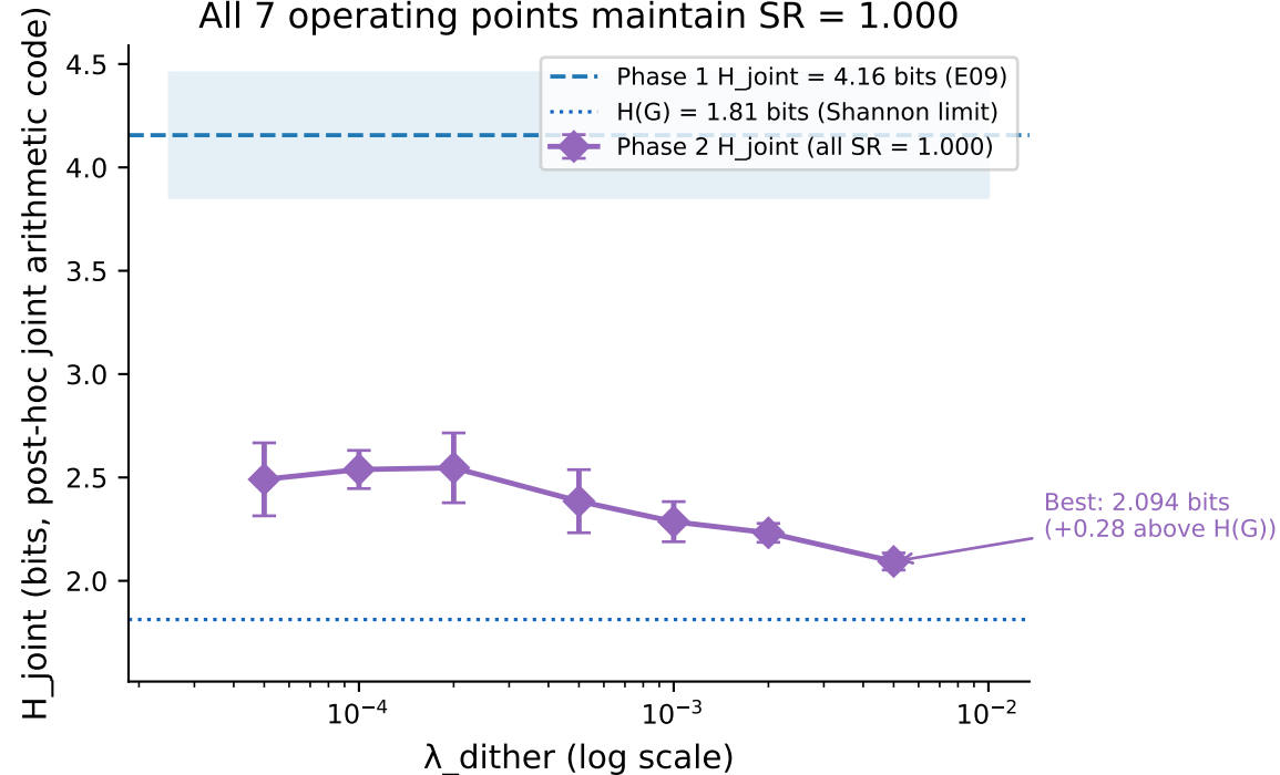
(A) Phase 2 compression curve: H_{\text{joint}} vs \lambda_{\text{dither}}
