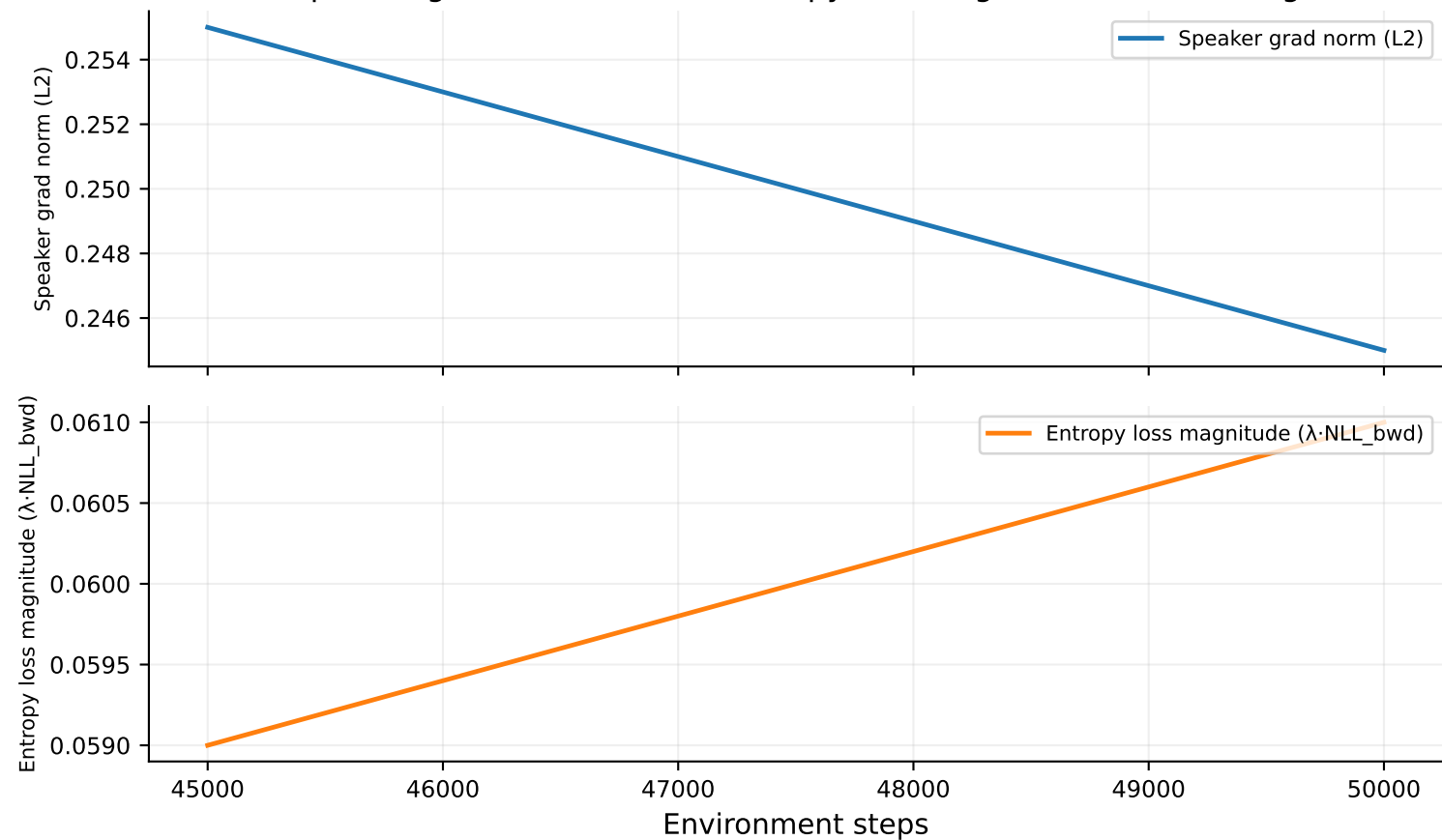
Speaker gradient norm and entropy loss magnitude over training
