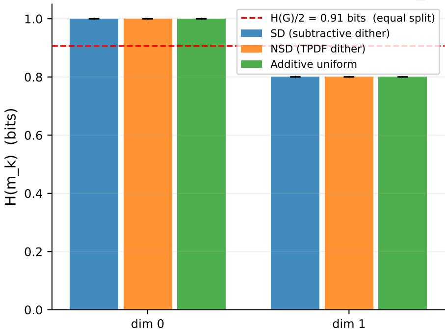
Per-dimension message entropy at convergence [z_dim=2]
