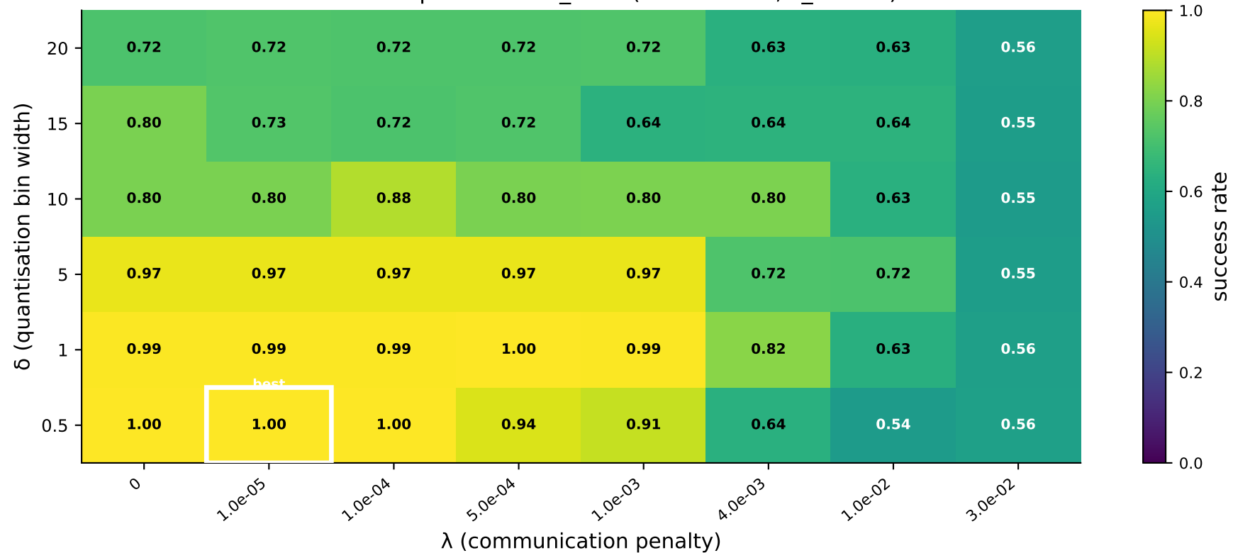
\delta \times \lambda heatmap — success_rate (channel=sd, z_dim=2)
