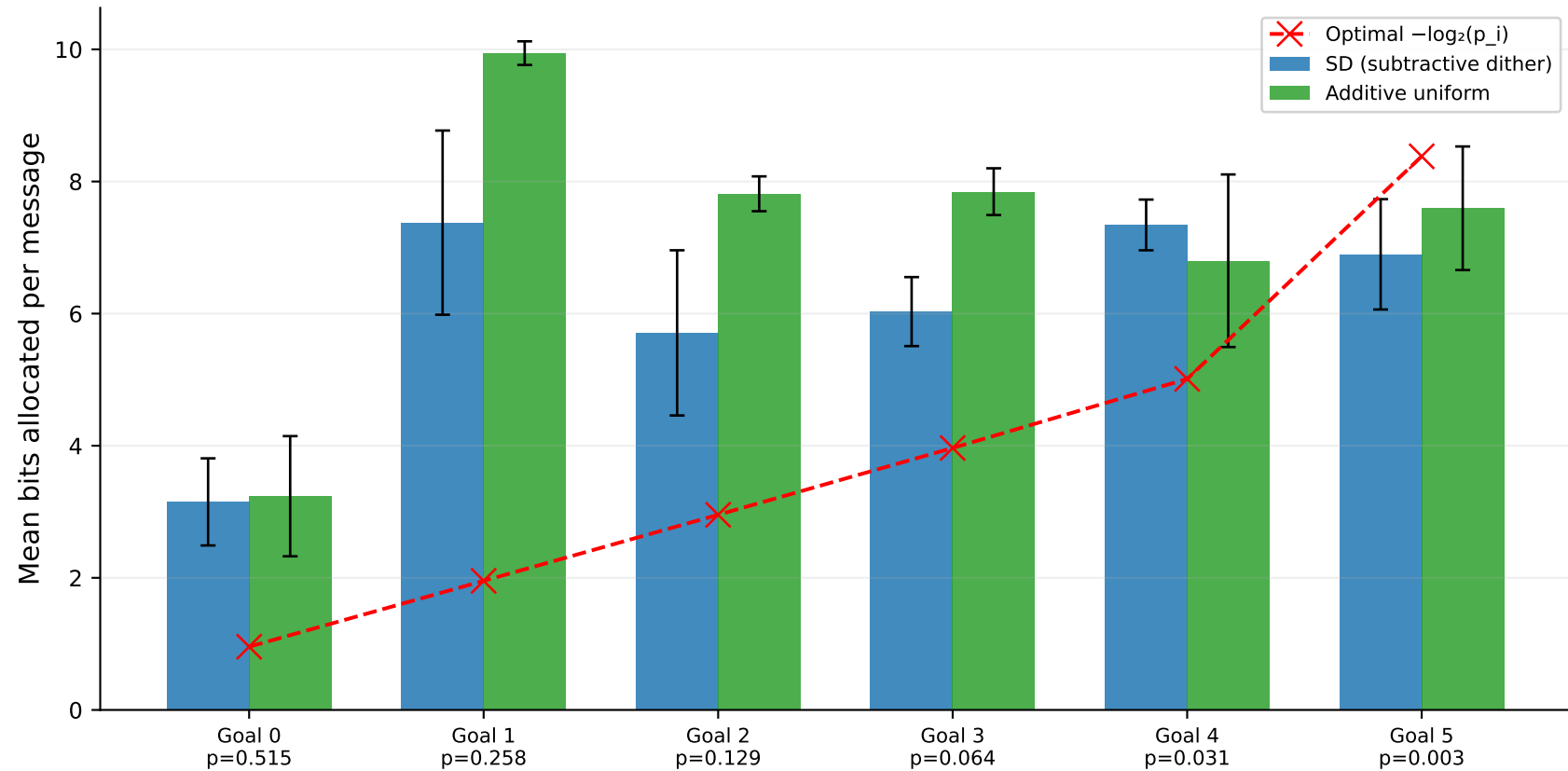
Per-goal bit allocation vs Shannon-optimal ( \delta=1.0 , \lambda=5.0\text{e-}04 , z_{\text{dim}}=2 )
