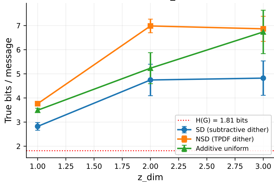
True bits vs z\_dim
