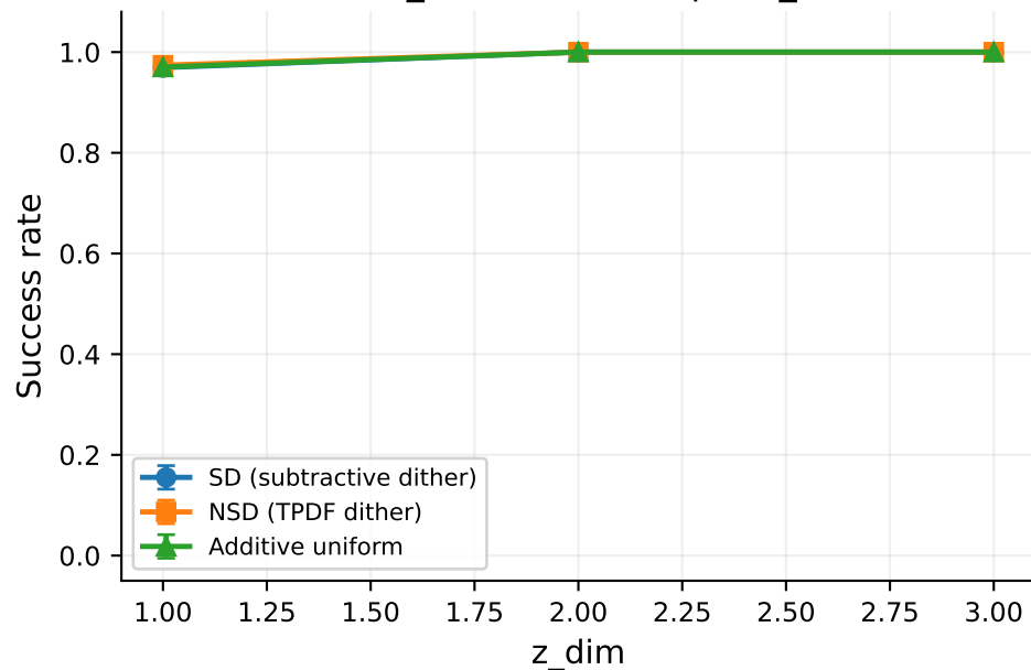
SR vs z\_dim (best \lambda , \delta per z\_dim )
