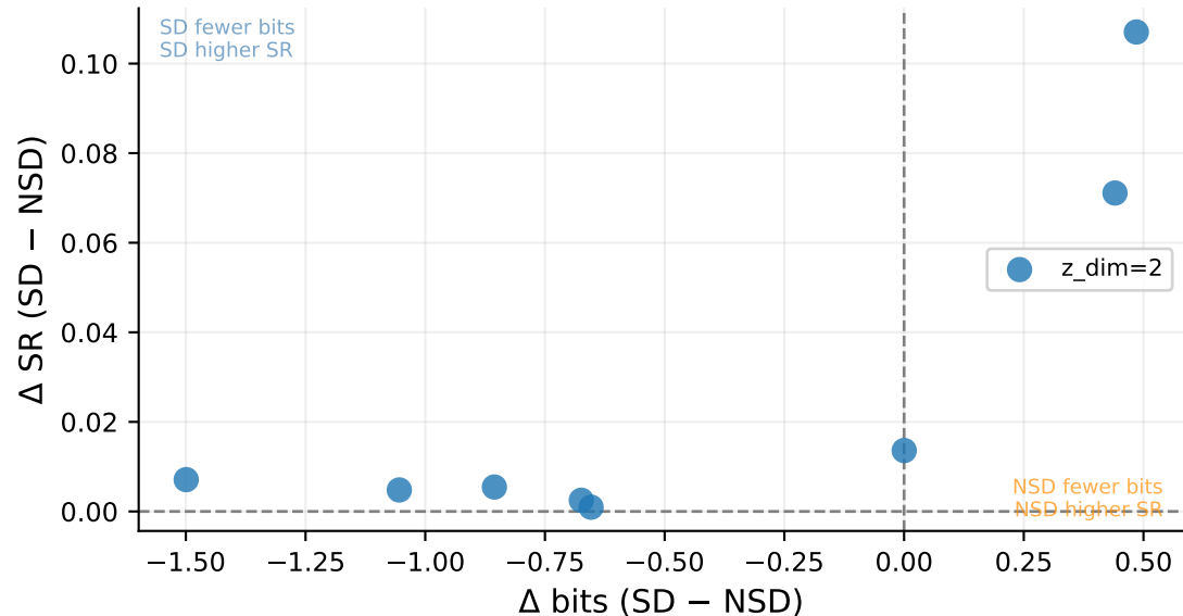
Per-config SD–NSD difference ( \delta=1.0 ) Upper-left = SD better on both metrics
