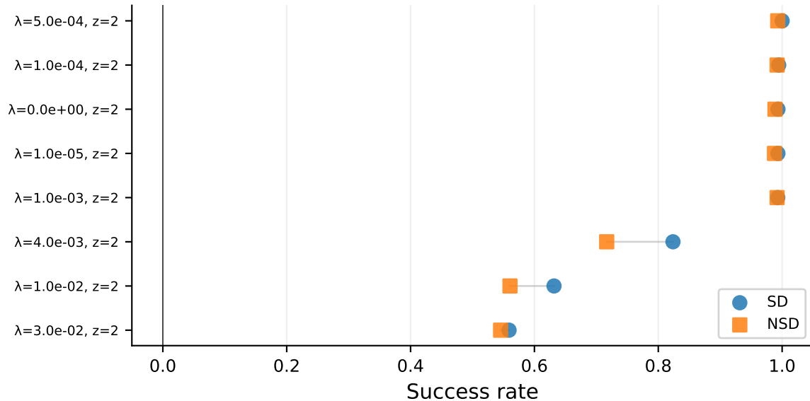
Paired SR: SD vs NSD ( \delta=1.0 ) Each row = one config; lines connect matched configs
