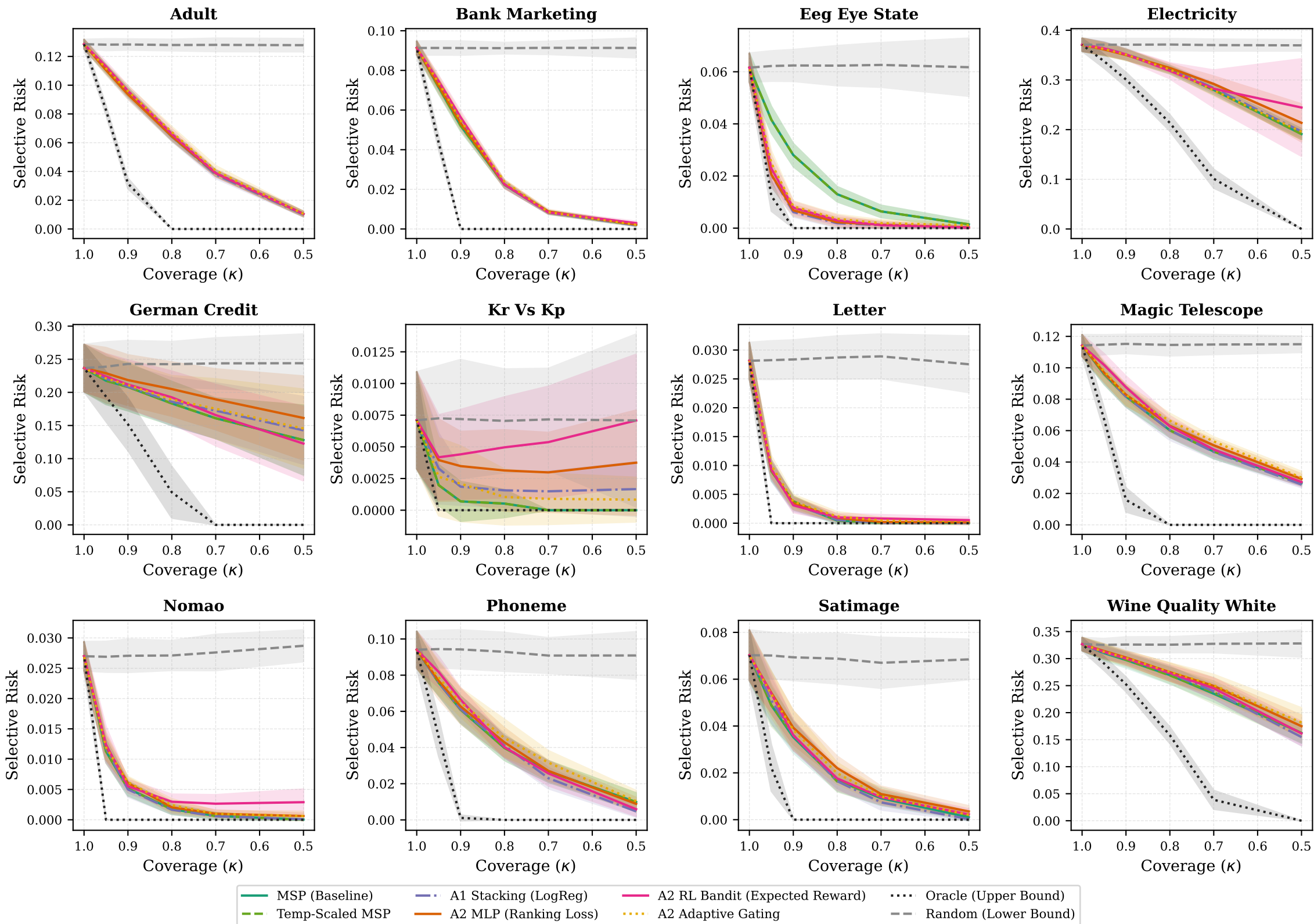
Selective Risk vs. Coverage Across Benchmarks (Tiers: ABC)
