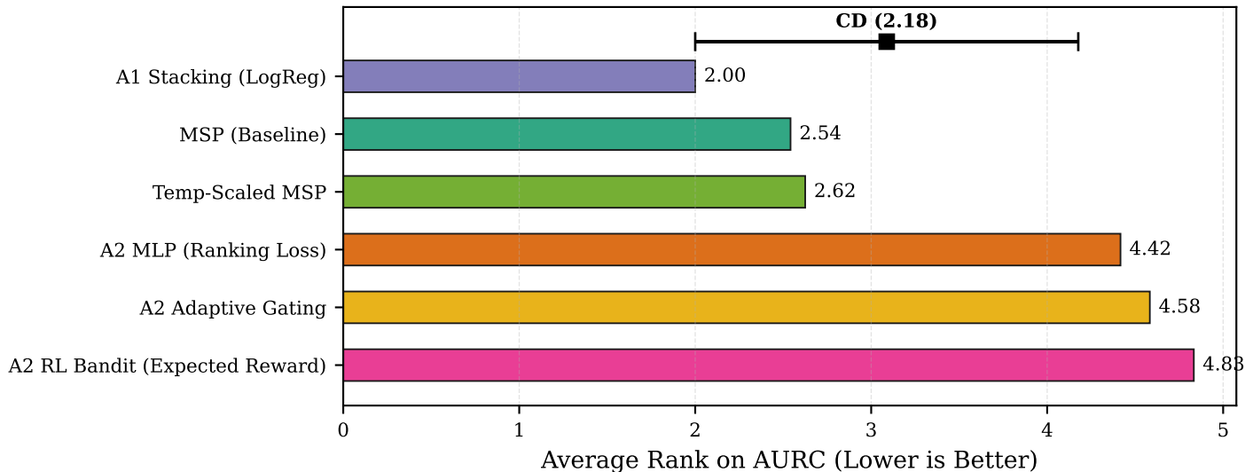
Friedman Mean Ranks & Critical Difference (Nemenyi CD = 2.18, N=12 Datasets)
